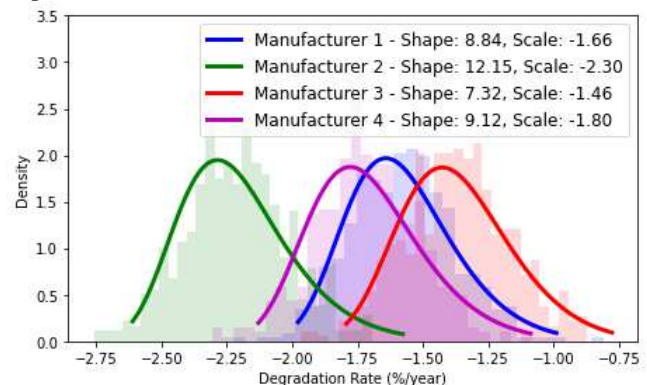
Fig. 2. Results of the G/tB PV systems degradation rate.
