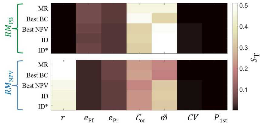
Figure 9. The effect of the uncertain factors (x-axis) is quantified with the total-order S_T sensitivity index (y-axis) based on robustness metric, RM_{PB} (first row) and RM_{NPV} (second row) and where dark gray is insensitive and white is sensitive.
