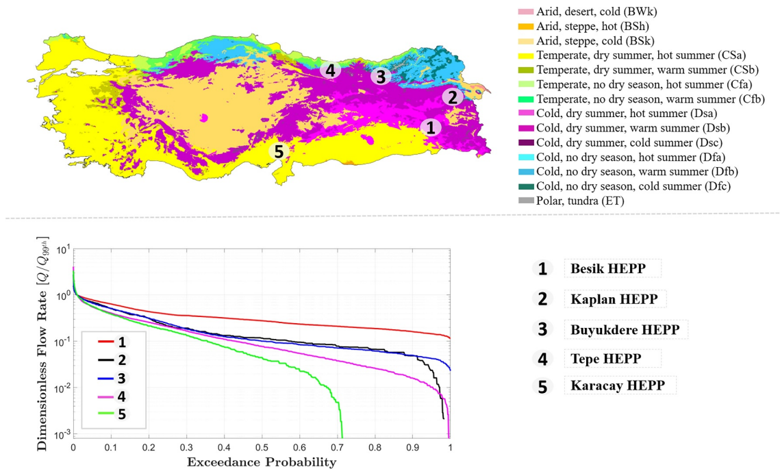
Figure 1. Top panel: Location of the presented five case studies on Köppen-Geiger climate classification map of Türkiye (Beck et al., 2018). Bottom Panel: Presenting Flow Duration Curves (FDC) for five case studies, where normalization is applied based on the 99th percentile of the flow. The FDC depicts graphically the relationship between the magnitude of the discharge (on y-axis) and its exceedance probability (on x-axis). The flow rate depicted on the y-axis is presented using a logarithmic scale.
