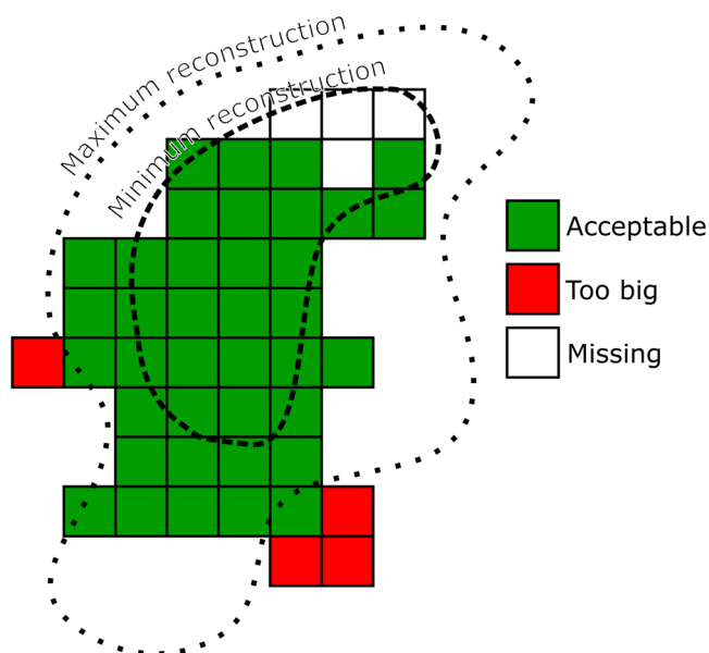
Figure 6. Overview of the 10 km model-data comparison procedure. A misfit score is calculated by summing modelled pixels that lie outside the empirically derived maximum limit ('too big') and those where ice is not modelled within the minimum empirical limit ('missing'). [Color figure can be viewed at wileyonlinelibrary.com ]
