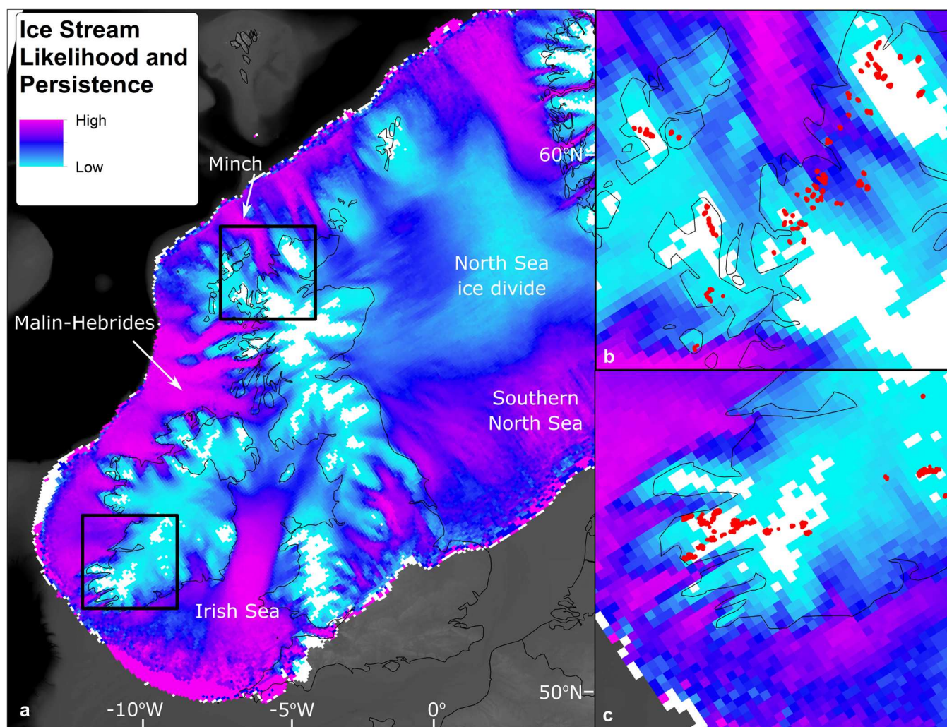
Figure 21. The location and persistence of fast flow. Fast flow was defined as regions of ice flowing above 100 \text{ m a}^{-1} . Values reflect the number of NROY simulations (likelihood) that produce ice stream flow for over 100 years (persistence), once the differing durations of ice cover each NROY produces are accounted for. (a) Overall persistence of ice stream conditions map. (b) and (c) show the locations of trimlines (Clark et al., 2018) in relation to ice streams. Note how many are co-located with regions of low ice stream persistence and likelihood. Overall, this map could be viewed as a proxy for glaciation-scaled erosivity and compared with the distribution and type of landforms such as tors, roches moutonnées, U-shaped valleys, bedforms, etc. Modern-day coastline is shown for orientation. [Color figure can be viewed at wileyonlinelibrary.com ]
