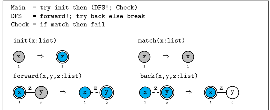
Fig. 1. The old program is-connected .
