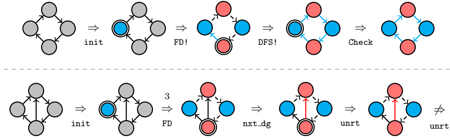
Fig. 7. Sample executions of 2-colouring on a 2-colourable (top) input graph and a non-2-colourable (bottom) input graph. FD , nxt_dg and unrt denote FORWARD , next_edge and unroot , respectively.
