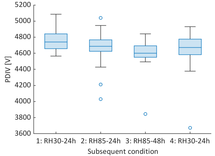
Fig. 9. Box chart of PDIV tests at each subsequent condition. Conditions are outlined in Table I.
