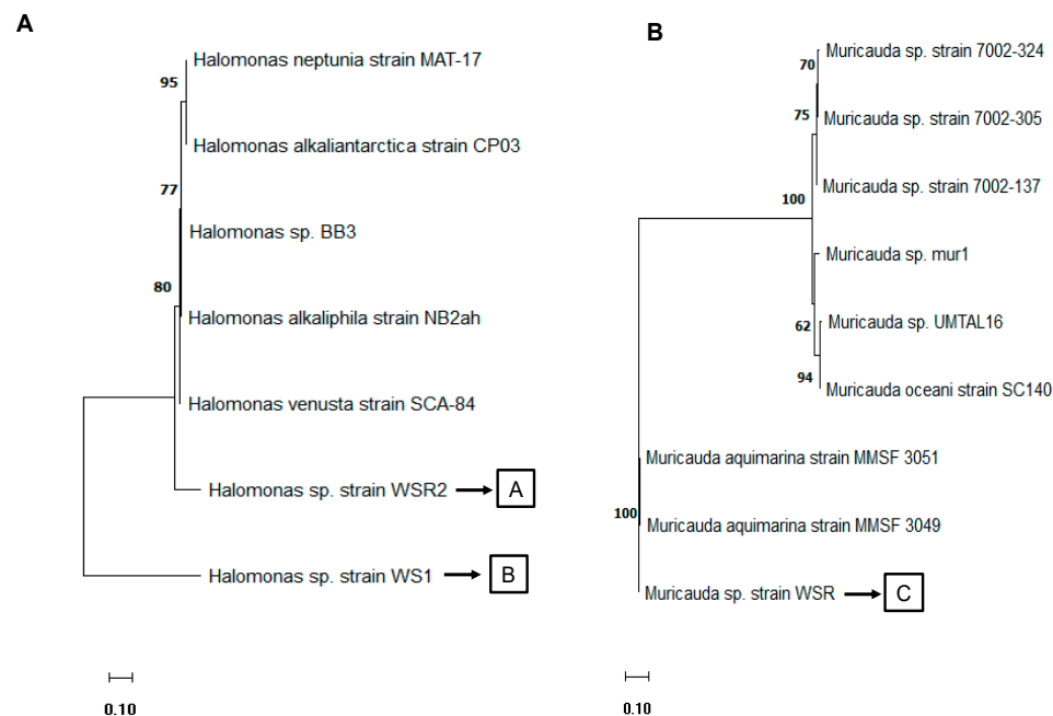
Figure 3. Phylogenetic tree of isolated cohabiting bacteria (A): Halomonas (A,B) and (B): Muricauda (C) from C. vulgaris culture and closely related species based on 16S rRNA sequencing, distance was estimated with Tamura-Nei model and branch support were assessed with 500 bootstraps using Mega 11.0 software.
