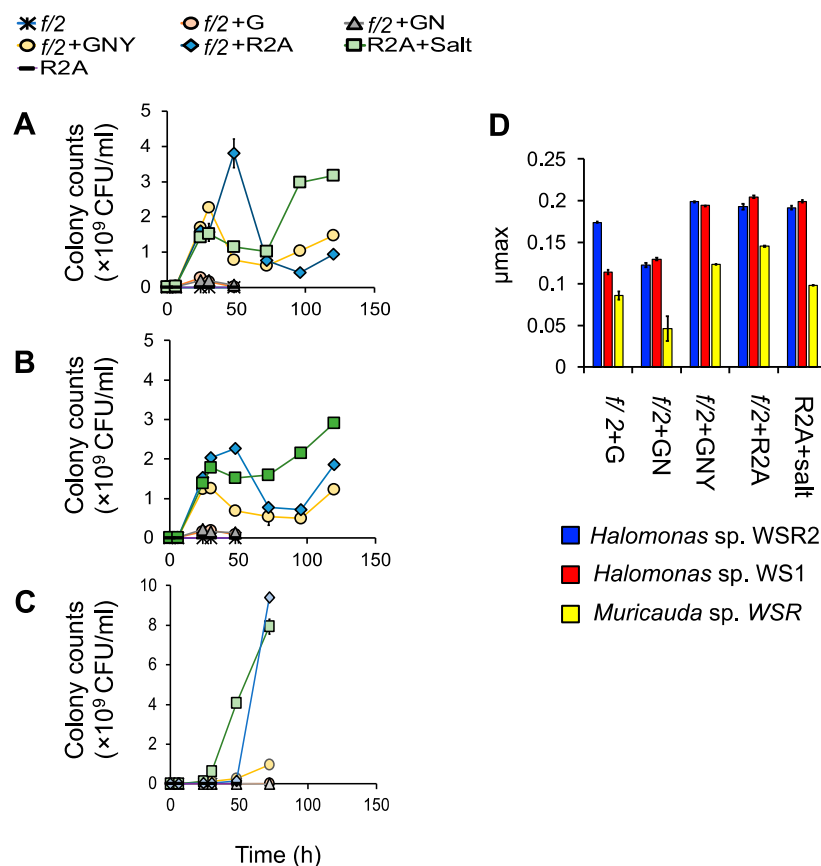
Figure 4. Growth rate by colonies count of bacterial isolates that grow in different media for optimal growth (A) Halomonas sp. WSR2, (B) Halomonas sp. WS1, (C) Muricauda sp. WSR, and (D) \mu_{\max} of the growth rate of all three species.
