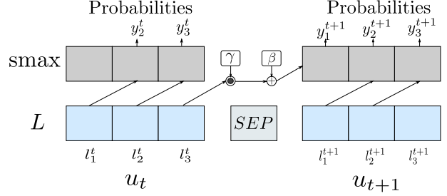
Figure 1: Modifications for language modelling in a conversational setting.
