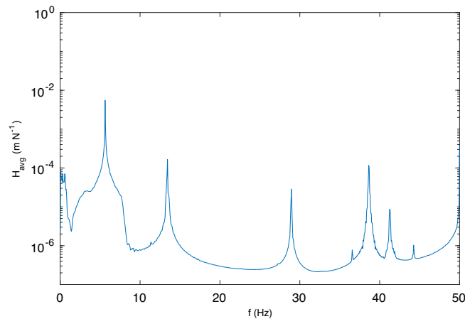
FIGURE 9 Average displacement FRF spectrum of the Garteur test structure, computed from the strain time histories using the iFEM approach, in the first damage condition analysed.
