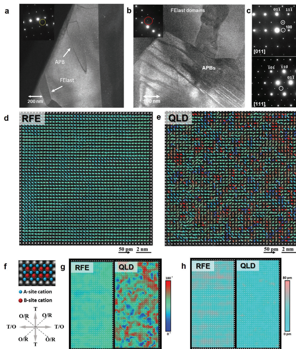
Figure 3. Advanced Transmission Electron Microscopy of RFE type NN-10ST-2LMT and QLD type \text{NN-Ta}_{0.10}\text{-10ST-2LMT} samples. a) DF image using a \frac{1}{2}\{\text{hk}0\} in phase tilt reflection and [001] zone axes from NN-10ST-2LMT superstructure reflections b) DF image using a \frac{1}{2}\{\text{hkl}\} antiphase tilt superstructure reflection, inclined to a \langle 110 \rangle zone axis showing antiphase boundaries in \text{NN-Ta}_{0.10}\text{-10ST-2LMT} . Ferroelastic domains are visible in the adjacent grain. c) [011] and [111] zone axes from NN-10ST-2LMT (equivalent patterns were obtained from \text{NN-Ta}_{0.10}\text{-10ST-2LMT} ). The ringed reflections in the [011] and [111] zone axes are at \frac{1}{2}\{\text{hkl}\} , \frac{1}{2}\{\text{hk}0\} , and \frac{1}{2}\{00l\} positions and are consistent with antiphase tilting, in phase tilting and antiparallel cation displacements, respectively. [55] The [001] -oriented atomic resolution HADDF-STEM images for d) NN-10ST-2LMT (RFE) and e) \text{NN-Ta}_{0.10}\text{-10ST-2LMT} (QLD). Individual arrows show B-site cation displacement vectors in individual unit cell with different vector angle. f) The blue and red spheres represent A- and B-site cations, respectively, and schematics of polarization directions for T, R and O structures are also shown. g) The projected polarization angle, and h) polarization magnitude mapping, derived from Figure 3d (RFE) and Figure 3e (QLD) and is indicated by contrast differences.
