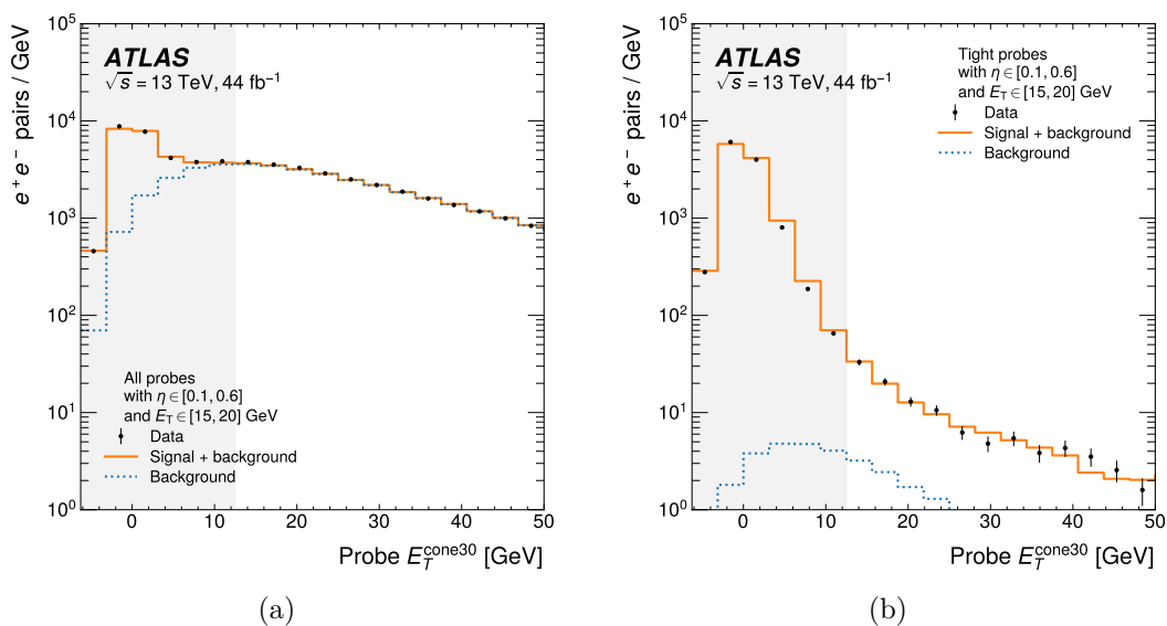
Figure 7. Examples of the probe E_T^{\text{cone30}} isolation variable distribution with the corresponding signal and background, using probes with \eta \in [0.1, 0.6] and E_T \in [15, 20] GeV. The nominal mass requirement m_{e^+e^-} \in [75, 105] GeV is already applied. The background template is normalised in the tail E_T^{\text{cone30}} > 12.5 GeV. The shaded area, E_T^{\text{cone30}} < 12.5 GeV, shows the nominal region used for efficiency extraction. (a) Including all the reconstructed probes, yielding the amount of signal in the denominator of the efficiency. (b) Including probes passing Tight identification, yielding the amount of signal in the numerator of the corresponding efficiency.
