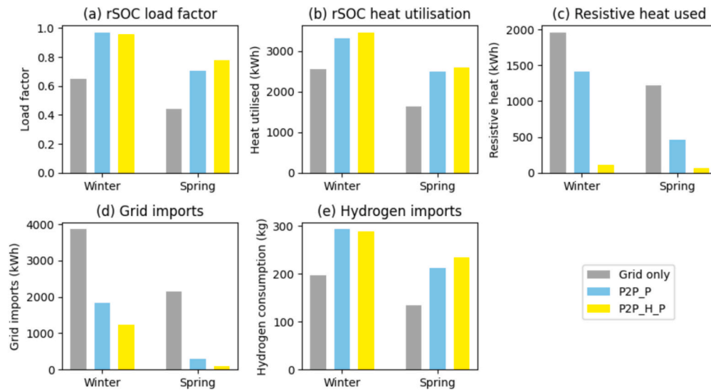
Fig. 12. Impact of P2P trading on various metrics: (a) Average load factor for SOFC mode over one week. (b) rSOC heat utilisation. (c) Resistive heat. (d) Grid imports. (e) Hydrogen imports.
