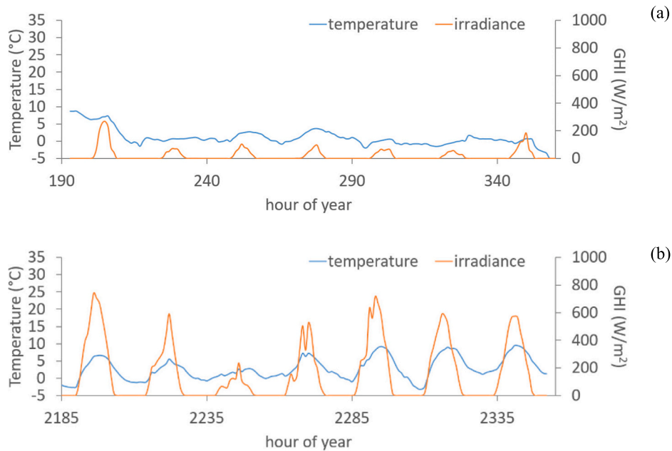
Fig. 4. Irradiance and temperature for (a) the winter week and (b) the spring week.
