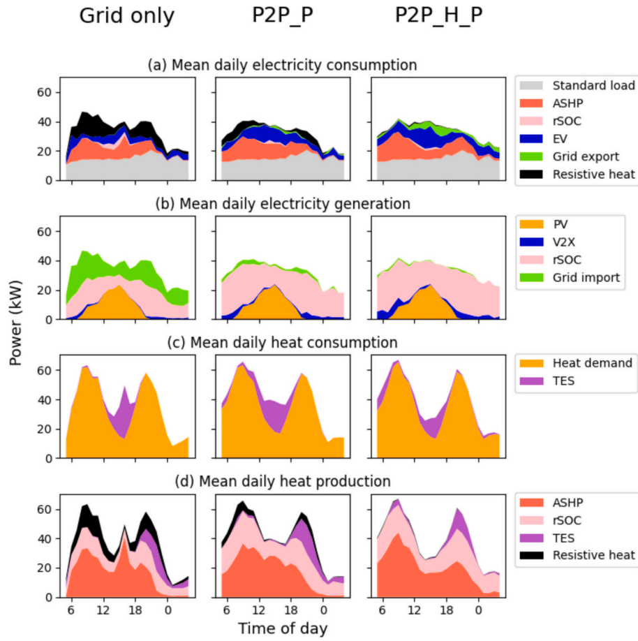
Fig. 9. Average daily energy flow during the spring week, for G_ONLY (left), P2P_P (centre) and P2P_H_P (right). Shown are the generation and consumption of both heat and electricity. Note that 5 a.m. corresponds to timeslot 0 in the market.
