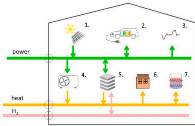
Fig. 3. Shows the possible devices included in houses (not all houses contain all devices). 1. PV generation. 2. EV. 3. Inflexible electric load. 4. ASHP. 5. rSOC. 6. Heat demand model. 7. TES. 25 houses with varying devices are included in the case-study.
