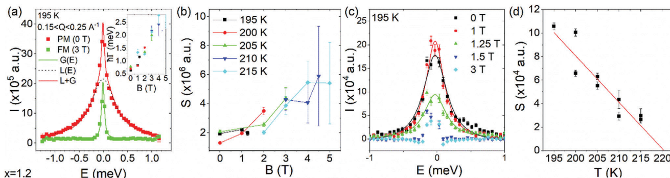
Figure 5. Summary of analysis of INS data obtained on LET, for E_i = 3.6 meV. a) Example linescans in the PM (0 T) and FM (3 T) state for 0.15 < Q < 0.25 \text{ \AA}^{-1} , alongside the pseudoVoigt used to determine linewidth shown in inset and integrated intensity, S , shown in (b). c) Example linescan for 0.48 \text{ \AA}^{-1} < Q < 0.56 \text{ \AA}^{-1} after background removal detailed in text. d) Corresponding integrated intensity, S , determined from fitting 0.48 \text{ \AA}^{-1} < Q < 0.56 \text{ \AA}^{-1} linescans at different temperature and fields where the QE feature was present.
