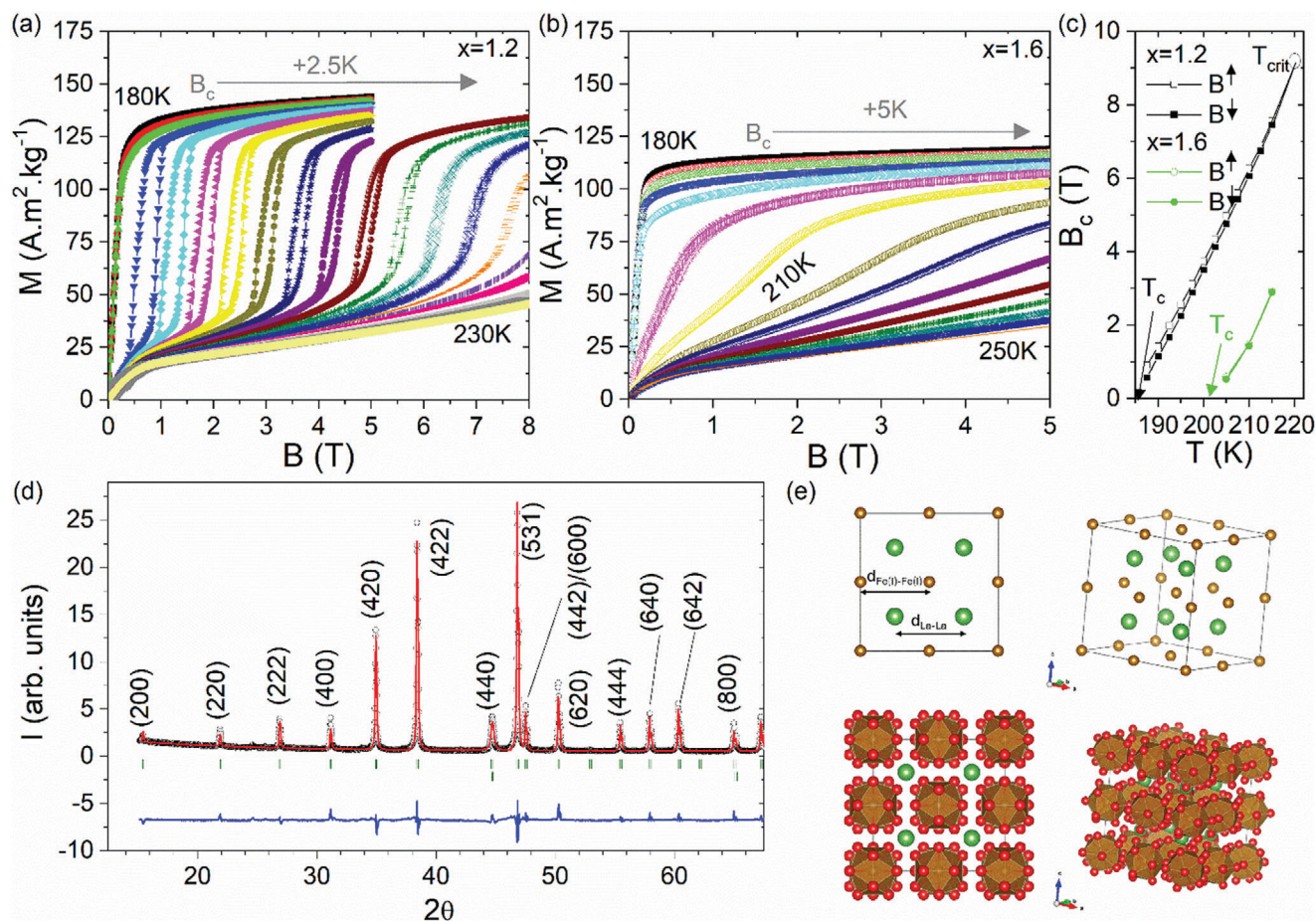
Figure 1. Summary of magnetization data for LaFe_{13-x}Si_x for a) x = 1.2 , and b) x = 1.6 at different temperatures. As the silicon content, x , is increased (or the temperature increased) the field driven phase transition broadens with an associated decrease in hysteresis. c) Magnetic phase diagram for each sample, where B^I is the field at which the magnetization has jumped to 50% of its saturation value from the paramagnetic state, and B^I is the point at which it falls to 50% of saturation value from its ferromagnetic state. Arrows indicate the Curie temperature, T_c , for each sample. d) Indexed x-ray diffraction data for x = 1.2 . The first observable Bragg peak was the (200) at 2\theta = 15.5^\circ . e) Schematic of the crystal structure. Top: 8a and 8b sites showing position of the Fe_I and La atoms. Bottom: full structure showing the icosahedral clusters of Fe_{II} that surround each Fe_I atom.
