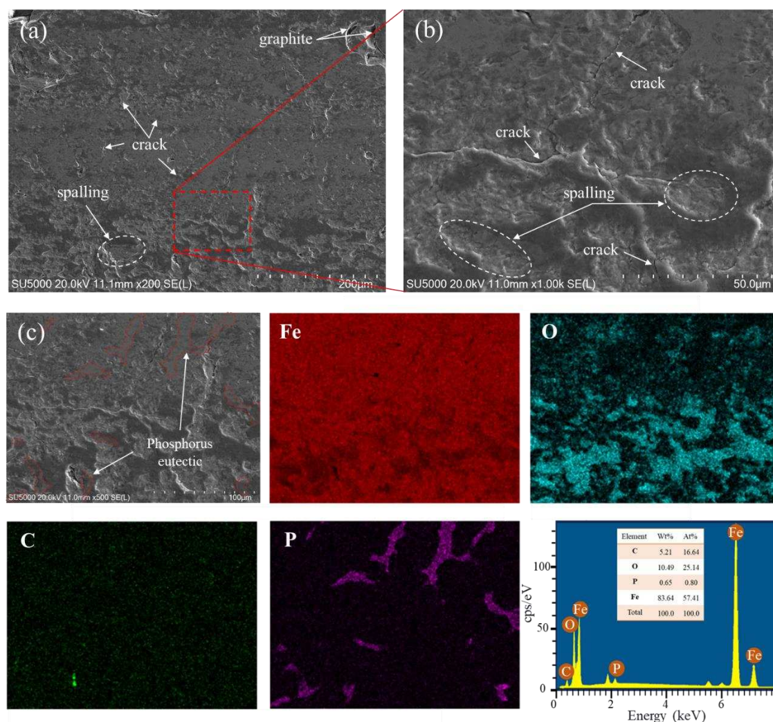
Fig. 13. Surface morphology and element distribution of wear scar when worn for 180 min: (a) surface morphology of wear scar, (b) local enlarged image, (c) local element
