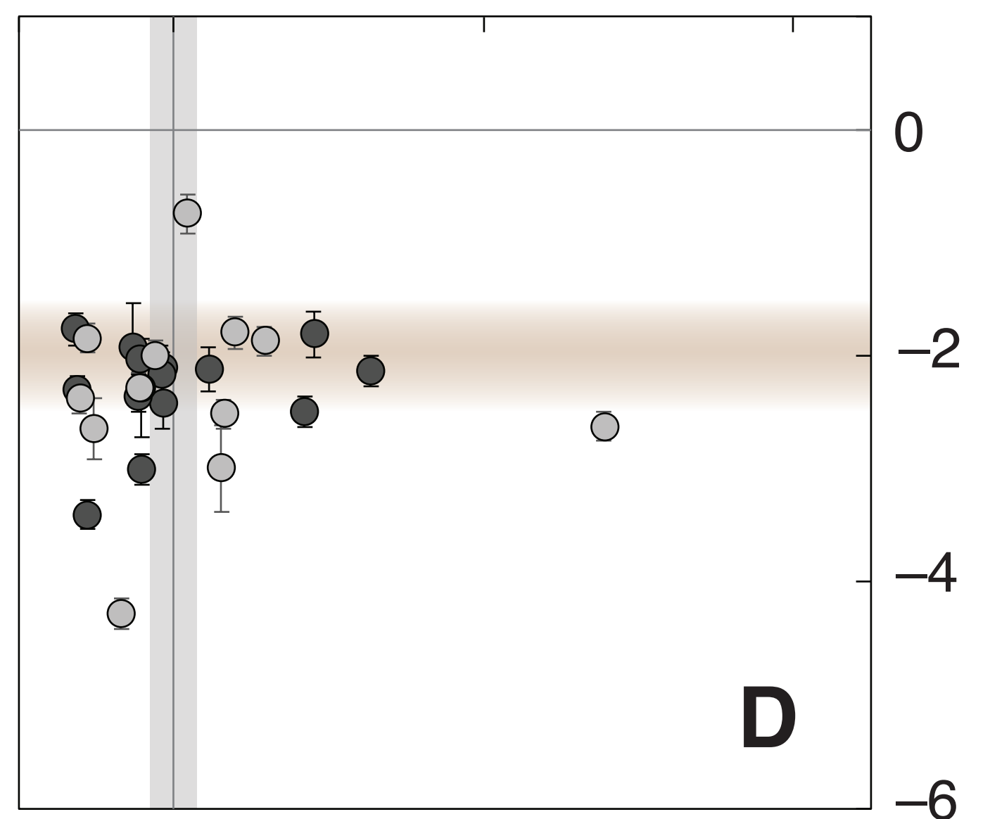
2.50 Ga old Mount McRae Shale (ABDP9 drill core)
