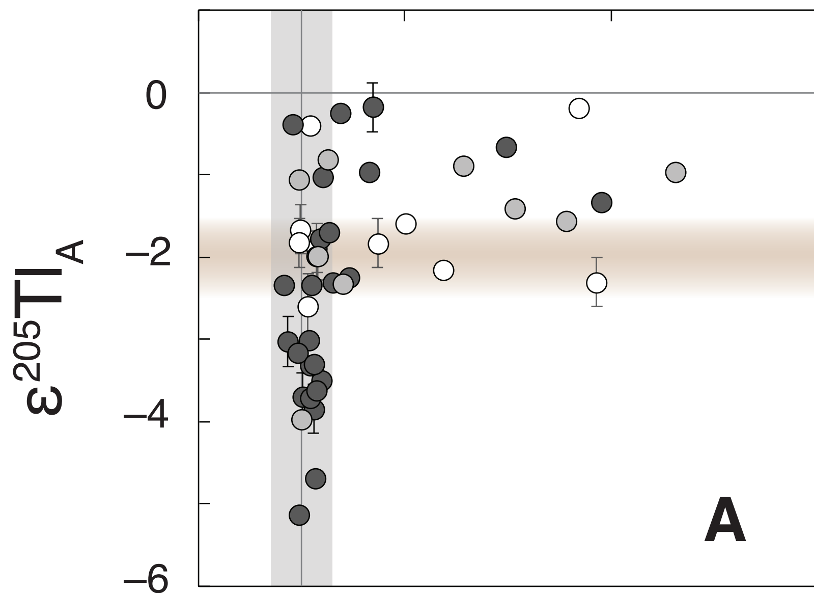
2.31 – 2.22 Ga old Rooihogte and Timeball Hill formations (EBA-2 drill core)
