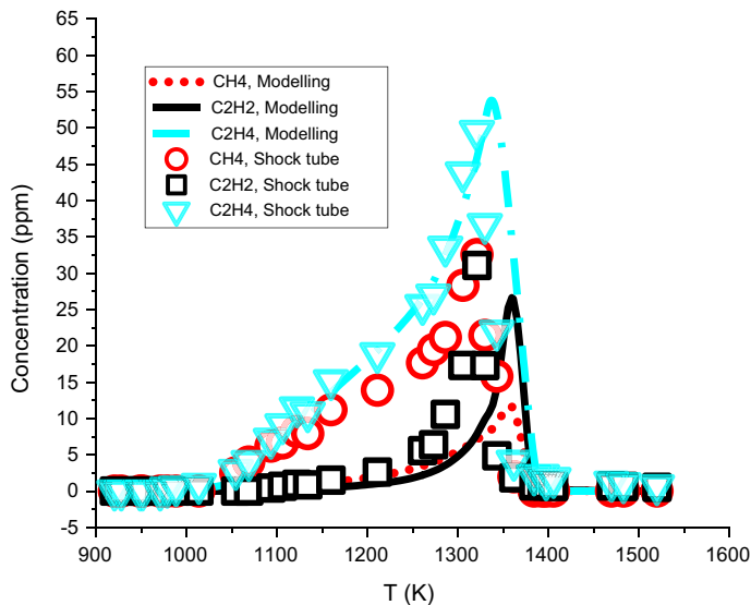
Fig. 5 Simulation results of CH 4 , C 2 H 2 , and C 2 H 4 concentrations for the developed mechanism of this study, against the low pressure shock tube experimental data for reaction time of 2.2 ms, at 4 bar over the temperature range of 900 to 1550 K [15]
