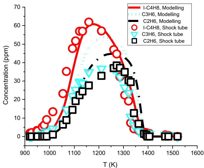
Fig. 4 Simulation results of I-C 4 H 8 , C 3 H 6 , and C 2 H 6 concentrations for the developed mechanism of this study, against the low pressure shock tube experimental data for reaction time of 2.2 ms, at 4 bar over the temperature range of 900 to 1550 K [15]
