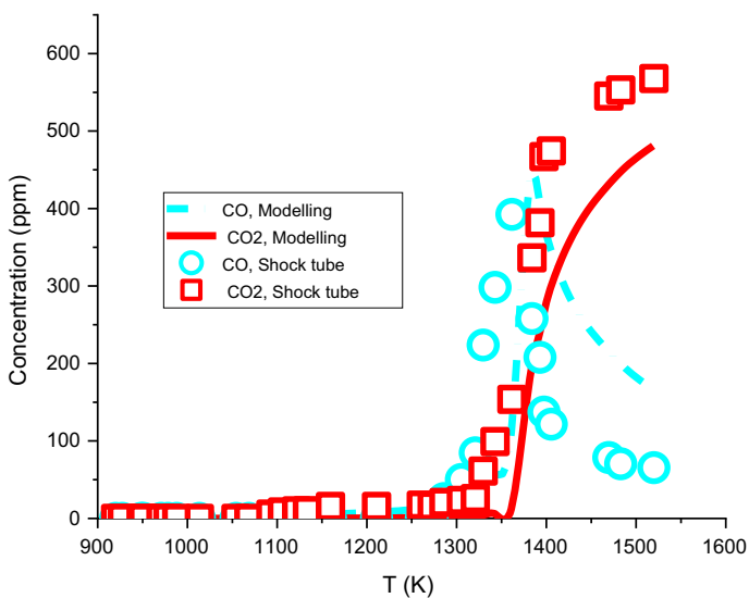
Fig. 7 Simulation results of CO and CO2 concentrations for the developed mechanism of this study, against the low pressure shock tube experimental data for reaction time of 2.2 ms, at 4 bar over the temperature range of 900 to 1550 K [15]
