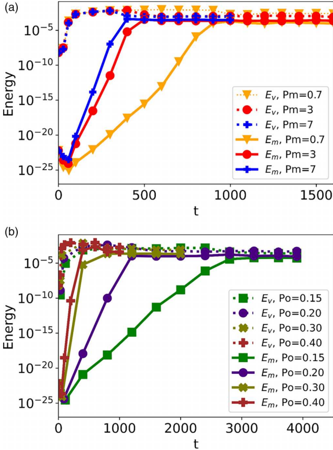
FIG. 1. Evolution of the volume-averaged kinetic \langle E_v \rangle (dotted) and magnetic \langle E_m \rangle (solid) energies at \text{Re} = 3 \times 10^4 for (a) different Pm at \text{Po} = 0.3 and (b) different Po at \text{Pm} = 3 . The magnetic field energy starts to grow after the saturation of the precessional instability and increases exponentially by several orders of magnitude, indicating an efficient dynamo action due to precession-driven turbulence.
