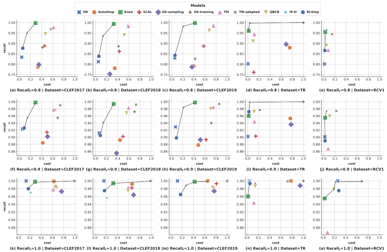
Figure 1: Performance of RLStop and baselines for Recall vs. Cost metrics. Grey lines indicates non-oracle Pareto optimal approaches. (Note differences in range of y-axis (recall) to avoid clustering of results.)
