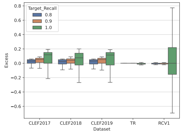
Figure 2: Distribution of RLStop excess across topics. (Outliers for target recall 1.0 removed for clarity.)
