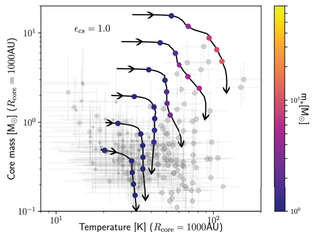
Figure E1. Core-fed models. Each track has been computed for a different initial core mass, from bottom to top m_{\text{core}}(t=0) = [0.5, 1, 2, 4, 8, 16] M_{\odot} . The coloured symbols represent the position of the cores at times t = [9 \times 10^3, 9 \times 10^4, 1.8 \times 10^5, 2.7 \times 10^5, 3.6 \times 10^5] yr. The colour codes the stellar mass at these times as displayed by the colour bar. The background grey symbols are the ArTéMiS sources whose properties have been rescaled to 0.01pc (see text). Note that sources with M_{\text{gas}} < \frac{1}{2} M_{\text{BE}}^{\text{crit}} have been removed.
