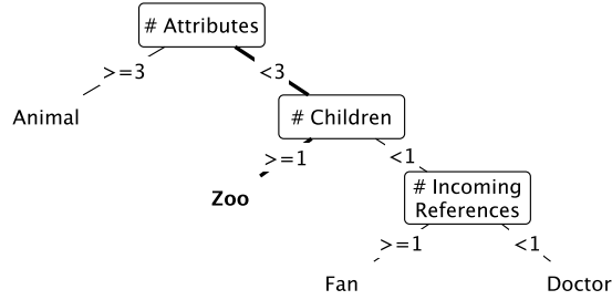
Fig. 5. Example Decision Tree
