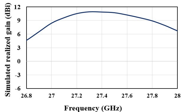
Fig. 4. Simulated realized gain of the proposed antenna array
