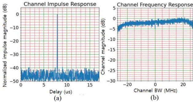
FIGURE 7. (a) Impulse response and (b) Channel frequency response in route A
