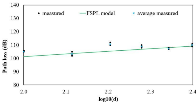
FIGURE 8. Extracted path loss of route A_elevated
