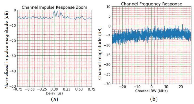
FIGURE 23. (a) Impulse response (b) Channel frequency response in route G at 80 m.
