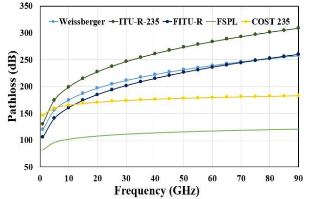
FIGURE 2. Comparison of the foliage path loss models with frequency at a fixed foliage depth of 300 m
