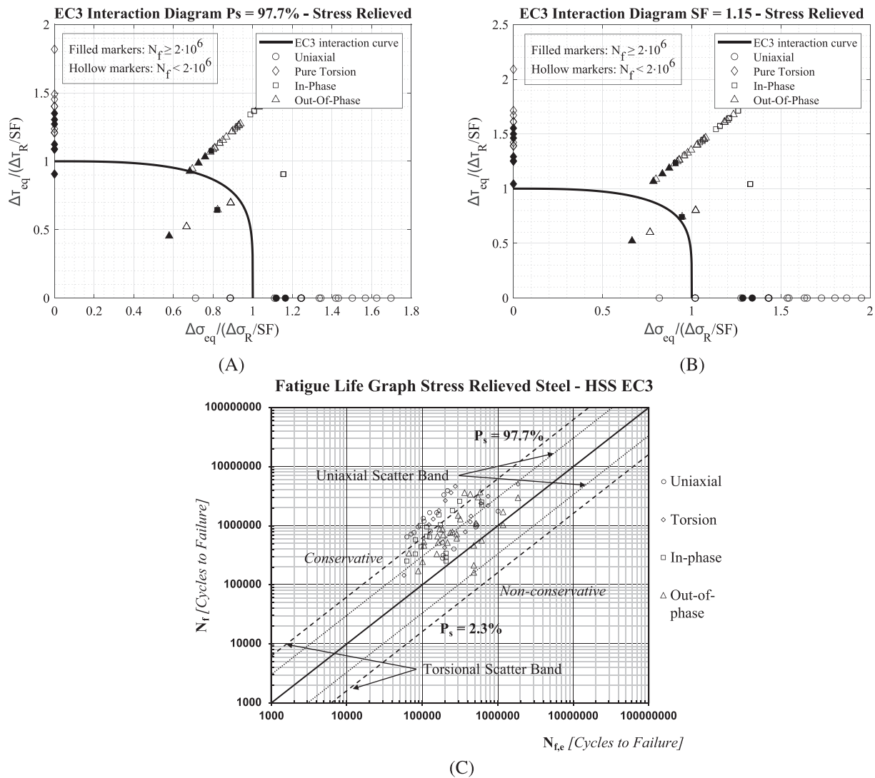
FIGURE 17 Hot spot stress (HSS) approach: EC3 interaction diagram (A, B) and fatigue life graph (C) for stress-relieved steel welded joints under VA fatigue loading, with reference stresses ( \Delta\sigma_R and \Delta\tau_R ) recalculated based on P_s = 97.7\% and SF = 1.15
