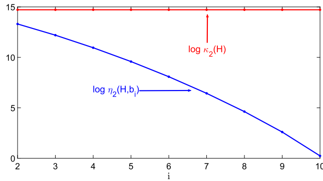
Fig. 1. The condition number \log_{10} \kappa_2(H) and effective condition number \log_{10} \eta_2(H, b_i) against i , for Example 2.2.
