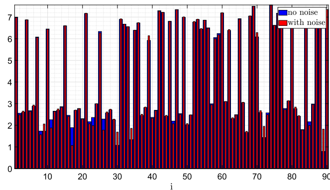
Fig. 11. The components \log_{10} |x_{1s,i}| of x_{1s} = A^\dagger b , with and without noise, for Example 5.3.
