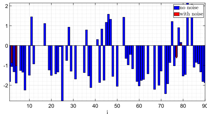
Fig. 4. The components \log_{10} |x_{\text{lasso},i}(\lambda^*)| of x_{\text{lasso}}(\lambda^*) , where \lambda^* is the optimal value of \lambda computed by 10-fold CV, with and without noise, for Example 5.1.
