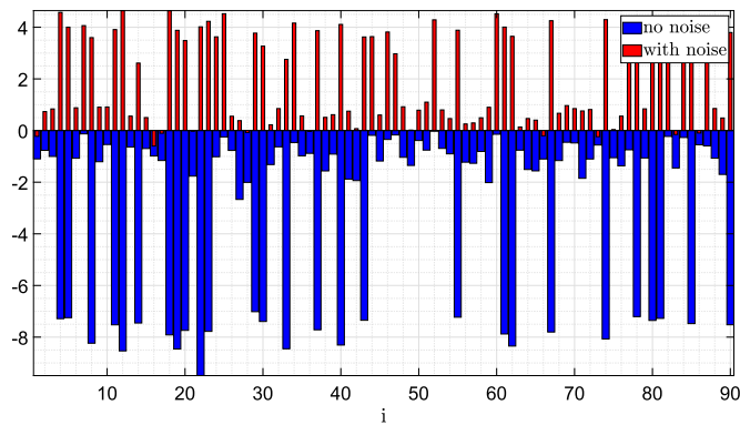
Fig. 3. The components \log_{10} |x_{1s,i}| of x_{1s} = A^+ b , with and without noise, for Example 5.1.
