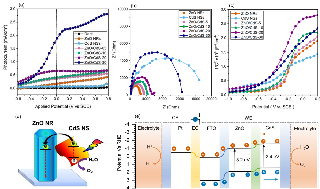
Figure 5. (a) Difference in photocurrent density as a function of the applied potential for ZnO-NRs, CdS-NSs, and ZnO/CdS hetero-structures prepared at different dipping durations (b) Nyquist plots obtained from the electrochemical impedance spectra of ZnO-NRs, CdS-NSs, and ZnO/CdS hetero-structures prepared at different dipping durations. The inset provides a depiction of the equivalent circuit model pertinent to the electrochemical impedance spectra. (c) Mott-Schottky curves of for ZnO-NRs, CdS-NSs, and ZnO/CdS nanostructures prepared at different dipping durations. (d) Schematic of CdS/ZnO nanostructures (e) Carrier Transport Mechanisms during the photoelectrochemical water splitting using CdS/ZnO nanostructures as photoelectrode under light irradiation.
