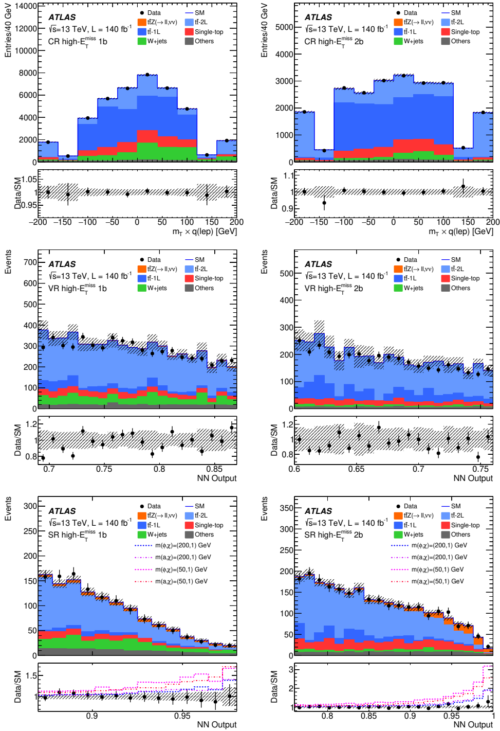
Figure 9. Observed and expected events as a function of m_T \times q(\ell) in the CR (top) and of the DM-NN output value in the VR (middle) and the SR (bottom) in the high- E_T^{\text{miss}} 1b (left) and 2b (right) DM regions. The expected distributions are as determined in the background-only fit with data in CRs and SRs for the t\bar{t} +DM search. The hatched area around the total SM prediction includes statistical and systematic uncertainties. Uncertainties on predictions in VRs are dominated by statistical uncertainties on simulated samples. The lower panels show the ratio of the observed data to the expected SM events, and the ratio of the sum of the SM and expected signal events to the SM events. In CRs, the last (first) bin contains overflows (underflows).
