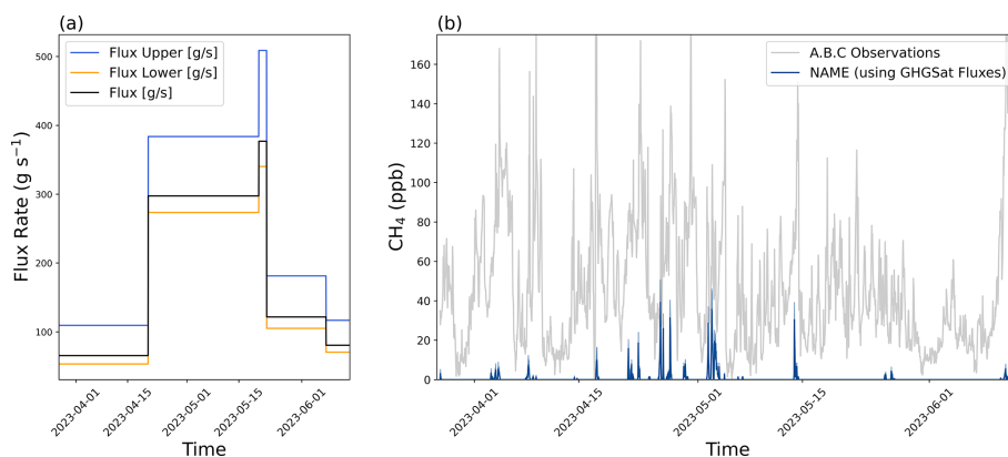
Figure 3. (a) Varying flux rates ( \text{g s}^{-1} ) used in the NAME model simulation “NAME-spring”. (b) Modelled \text{CH}_4 concentrations (ppb) at the Ridge Hill (RGL) tall tower site from GHGSat-derived flux rates in the NAME-spring simulation (blue) and observed above-background concentrations (A.B.C) at RGL (grey).
