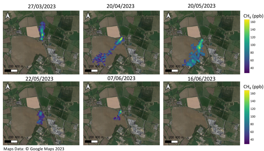
Figure 1. Total column \text{CH}_4 (ppb) observations from GHGSat showing the variation in strength and size of the plume from the gas leak on six dates between March and June 2023 (© Google Maps 2023). The geographical area shown is not the full field of view of the satellite and contains only the area where enhanced \text{CH}_4 concentrations were identified.
