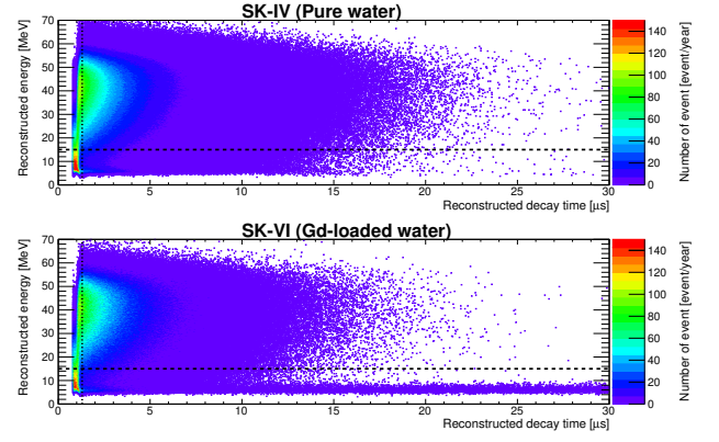
FIG. 29. The time difference between the stopping decay muon and the reconstructed events in the SK-IV (top) and -VI (bottom) data sample. In the SK-VI data sample, 8 MeV \gamma -rays originating from the neutron capture by gadolinium in water are observed after tagging the decay electron.
