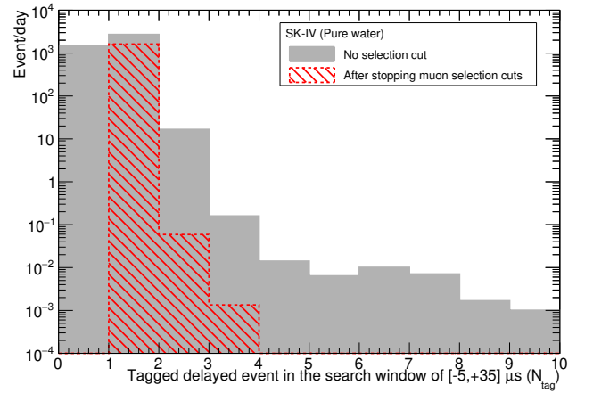
FIG. 16. The typical distribution of N_{\text{tag}} , which is defined as the number of tagged delayed events associated with single cosmic-ray muons, using the SK-IV data. The gray filled histogram (red left slanting histogram) show the number of events without (with) the selection cuts described in Sec. IV B 2.
