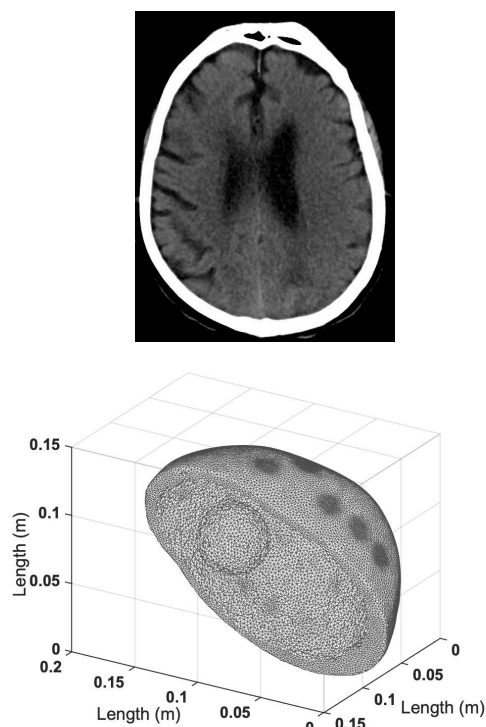
Fig. 4. Top: All the simulated anatomies are derived from CT neuroimaging of stroke patients. A sample CT slice of the anatomy used to create the fine mesh is shown (from resources supplied in [3]). Bottom: Fine mesh with 50 ml simulated spherical lesion in the north-east position (where the front of the head represents north). The brain layer has been removed in order to show the lesion. The electrode refinement on the scalp layer is also clearly seen.
