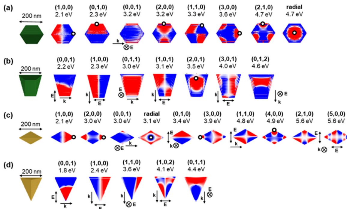
Fig. 2 Calculated near-field charge distribution of resonant modes in tent and kite shapes of Mg NPs. Plasmon modes of (a) tent, (b) filled tent, (c) kite and (d) filled (1121) kite where blue and red colours (arbitrary intensity) correspond to opposite charges on the NP's surface. Electron beam excitation is denoted by a black circle at the beam position, with propagation perpendicular to the page, while for photon excitation, the incident field direction ( k , single arrow) and polarisation ( E , double arrow) are shown. Incident field directions and polarisations perpendicular to the page are denoted with \otimes and a k or E annotation.
