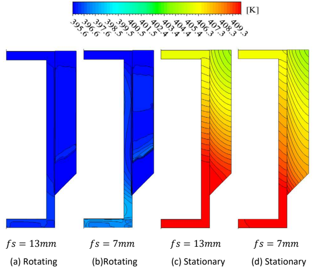
Fig. 4. Thermal contour distributions across the heat sink fin surfaces under static and rotating conditions for f_s = 7\text{mm} and f_s = 13\text{mm} .
