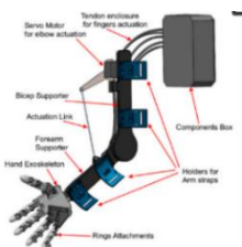
Fig 3.1 Arm and hand exoskeleton.
