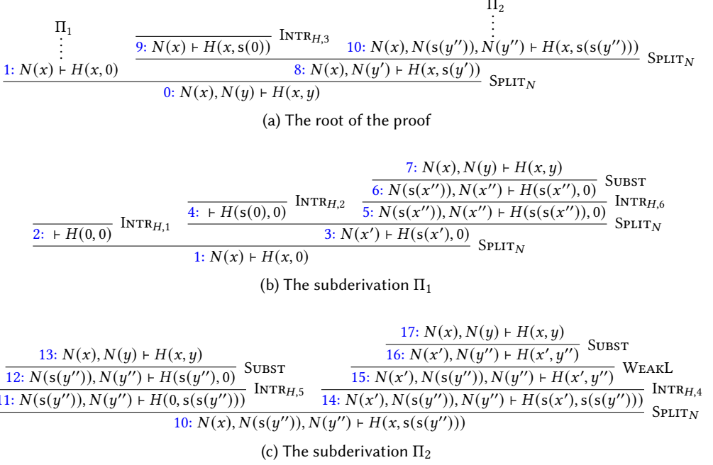
Fig. 2. A cyclic preproof in \text{LKID}^\omega(\text{Hydra}) of the totality of the 2-Hydra predicate.
