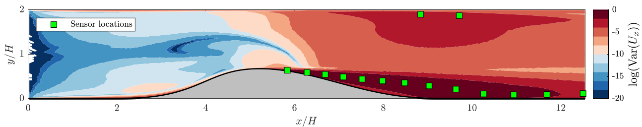
FIG. 19. The streamwise velocity uncertainty map for the converging-diverging channel.
