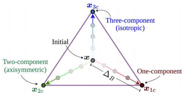
FIG. 2. Barycentric triangle used to perturb eigenvalues to their three limits. Mapping turbulence states on the Barycentric map is useful as Banerjee et al. 43 showed that all realizable turbulence states are bounded and presented by the edges and vertices of the equilateral triangle. In eigenspace perturbations an arbitrary Reynolds stress state \mathbf{x} is sequentially perturbed from the initial state to the three vertices \mathbf{x}_{1c} , \mathbf{x}_{2c} , and \mathbf{x}_{3c} .
