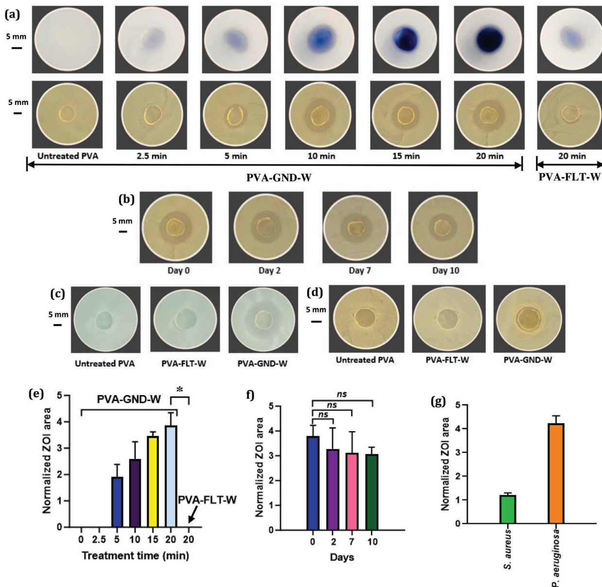
Figure 7. a) Photographs of color intensity (RONS transfer) produced in the agarose containing the by KI-starch RONS reporter dye (top row) and corresponding photographs of E. coli ZOI (bottom row) for different plasma treatment times of PVA-GND-W hydrogels and the PVA-FLT-W hydrogel plasma treated for 20 min; quantified ZOI is shown in (e) ( n = 6 ). b) photographs and f) quantified E. coli ZOI produced by 20 min plasma treated PVA-GND-W hydrogels freshly prepared (day 0) and following storage for 2, 7, and 10 days ( n = 3 ). Photographs of c) P. aeruginosa and d) S. aureus ZOI and g) quantified ZOI for both bacteria produced by freshly prepared 20 min plasma treated PVA-GND-W hydrogels ( n = 3 ). Photographs of the of the petri dishes with PVA hydrogel on top are shown in Figures S2–S6 (Supporting Information). Data are presented as mean \pm standard error of the mean (SEM). * p < 0.0001 , ^{ns} p > 0.05 (Student t -test). ns = not significant.
