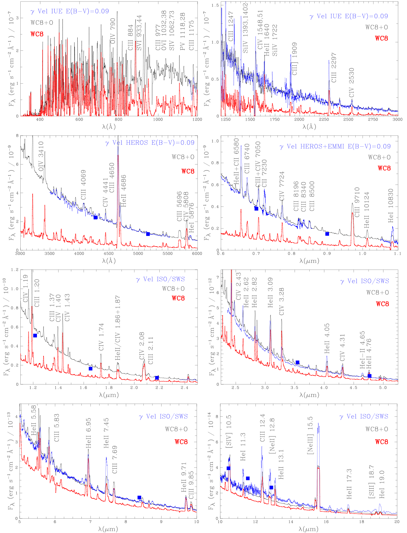
Figure 4. De-reddened UV IUE/HIRES spectroscopy (phase 0.5), calibrated optical ESO 50cm+HEROS and NTT+EMMI He I \lambda 10830 spectroscopy, ISO SWS infrared spectroscopy of \gamma Vel (blue), together with theoretical WC8+O model (black) and WC8 component (red), excluding correction for interstellar H I. Optical-IR photometry (Johnson et al. 1966; Williams et al. 1990; De Marco et al. 2000; Wright et al. 2010) is presented as blue boxes.
