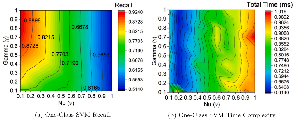
Fig. 3. One-Class SVM (OCSVM).
