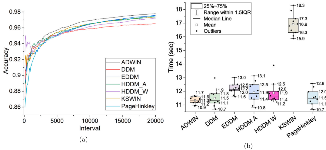
Fig. 7. Comparison of Concept-drift Detection methods.
