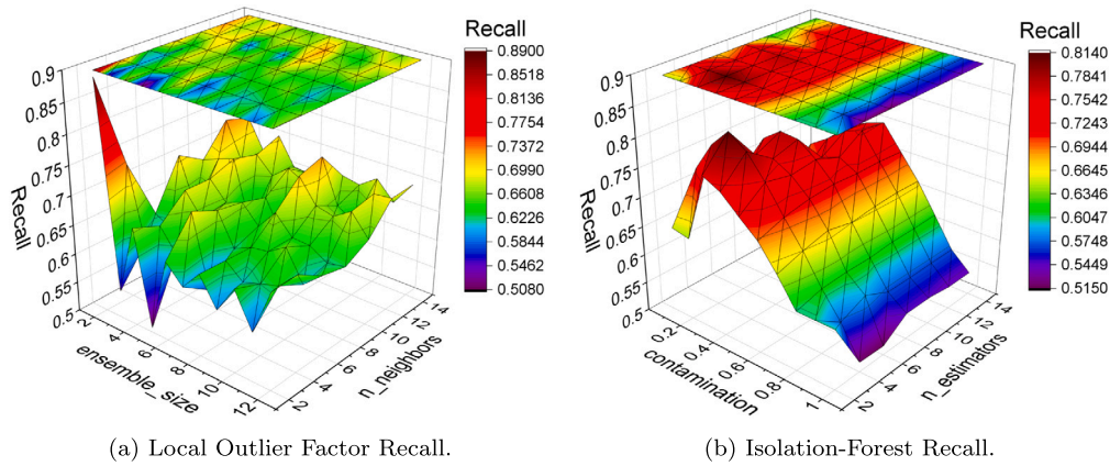
Fig. 4. Performance of different outlier detection algorithms.
