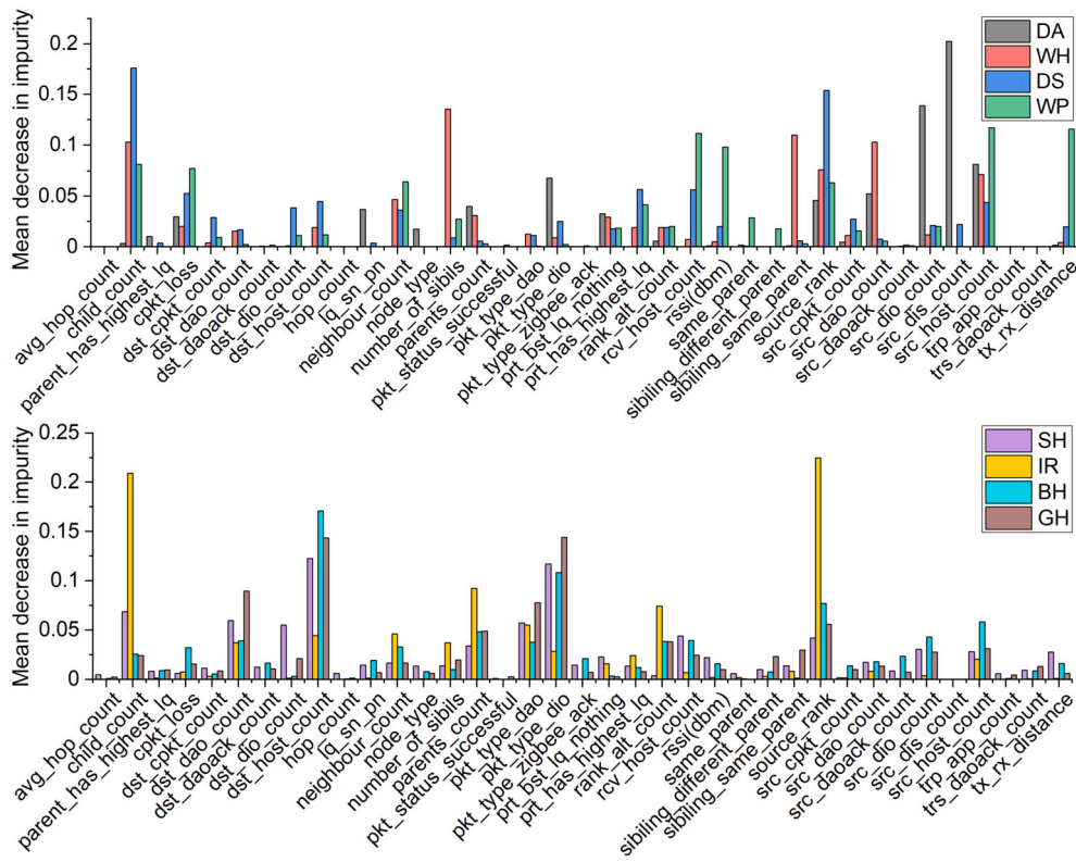
Fig. 2. Feature importance.
