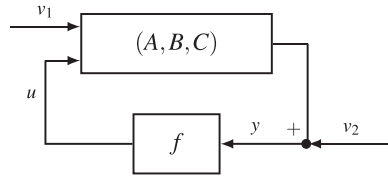
FIG. 1. Block diagram of forced Lur'e system (1.1).
