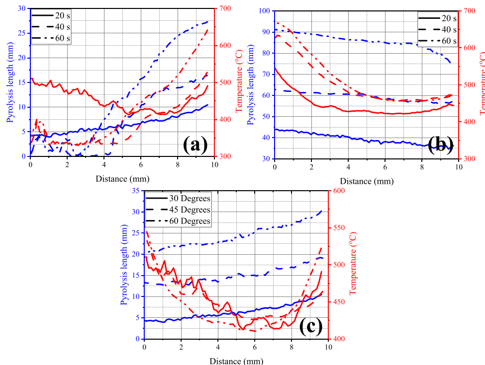
Fig. 10. Side surface pyrolysis length ( T > 300^\circ\text{C} ) and the average temperature of the pyrolysis region as a function of the distance to the bottom of the sample (demonstrated in Fig. 3 (b)). (a) Bottom surface coated sample inclined at 30 degrees. (b) Top surface coated sample inclined at 30 degrees. And (c) Bottom surface coated sample at different inclination angles ( t = 20 s).
