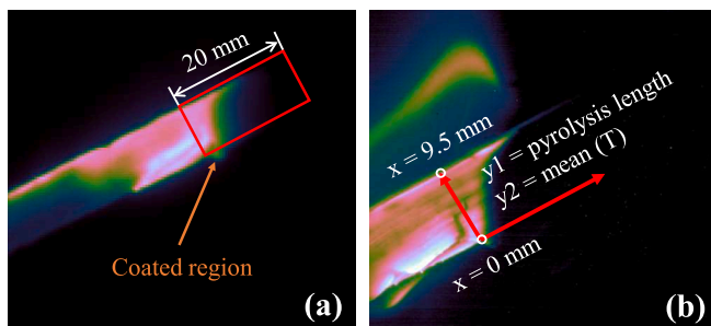
Fig. 3. Illustration of the region of interest (ROI). (a): The temporal mean temperature of LWIR camera. (b): The spatial distributions of the pyrolysis zone in the coated region of InGaAs SWIR camera.
