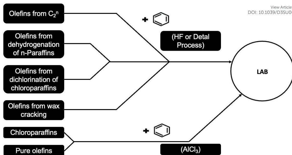
Figure 5 - the most common LAB production methods (adapted from Shokri and Karimi). 3
