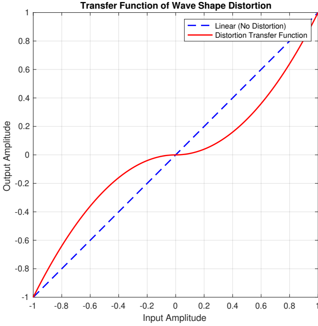
Fig. 4. Transfer function of a full-range distortion wave shaper. This graph illustrates the nonlinear mapping of input amplitudes to output amplitudes, with the red line depicting the distortion transfer function and the blue dashed line representing the linear undistorted signal.
