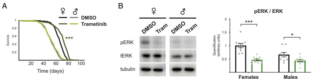
Fig. 1. Trametinib extends lifespan in females but only sometimes and to a much lesser extent in males. (A) Survival curves showing trametinib significantly extends female lifespan ( P = 2.06 \times 10^{-12} ***; n = 150 ; log-rank test) and does not extend male lifespan ( P = 0.36 ; n = 170 ; log-rank test), representative of the seven trials. Trametinib feeding significantly extended female lifespan in all seven trials, while it did not extend male lifespan in five out of seven trials (see SI Appendix, Fig. S1 for representation of all the trials performed). (B) Trametinib feeding significantly decreased pERK levels in the gut compared to Dimethyl sulfoxide (DMSO)-fed flies (control), both in females (Welch's t test, P < 0.0001 ***) and males (Welch's t test, P = 0.039 *). Western blot (Left) and quantification of the bands (Right) showing the ratio pERK/ERK after normalization with Tubulin. Bar charts show mean \pm SEM, n = 9 to 10 biological replicates per condition with 5 guts per replicate.
