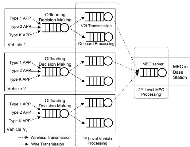
Fig. 2: Model abstraction for VEC systems
