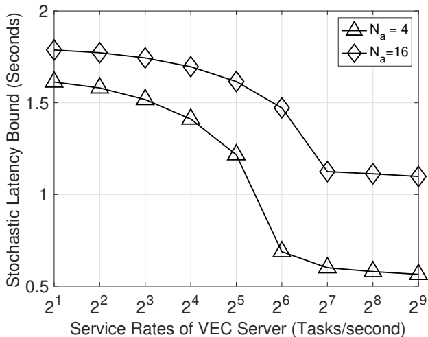
Fig. 9: Impact of the VEC service capabilities on the stochastic latency bound with \varphi_{1,n,k} = 0.7 , \varphi_{2,n,k} = 0.35 , \lambda_{n,k} = 24 , Nc_n = 6 , N_a = \{4, 16\} , \mu_{d,n}=40 , \mu_{vp,n} = 50 , \mu_{es} = \{2^1 - 2^9\} , V = 15 , \eta = 0.3 , \theta = 0.25 , \xi = 0.45 , K_{d,n} = 16 , K_{vp,n} = 16 , K_{es} = 32 .
