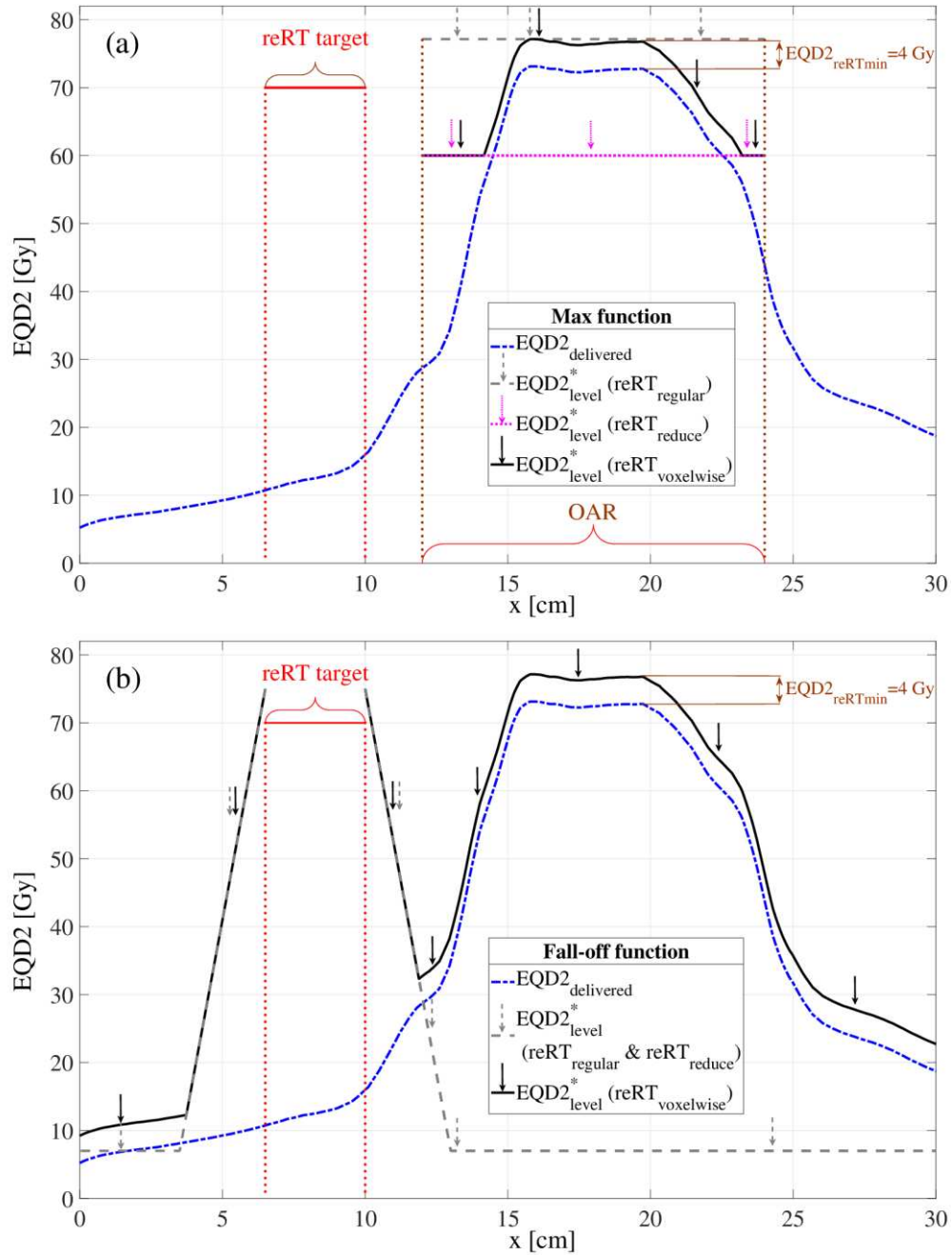
Figure 1. Schematic 1D illustrations of the adjusted equivalent dose in 2-Gy fraction (EQD2) penalization levels ( \text{EQD2}_{\text{level}}^* ) with an additionally allowed unpenalized re-irradiation (reRT) EQD2 ( \text{EQD2}_{\text{reRTmin}} ) of 4 Gy used in the planning of \text{reRT}_{\text{regular}} , \text{reRT}_{\text{reduce}} and \text{reRT}_{\text{voxelwise}} . (a): a maximum EQD2 function with \text{EQD2}_{\text{level}} of 60 Gy for an organ at risk (OAR) and (b): a EQD2 fall-off function linearly decreasing from 75 Gy at the reRT target edge to 7 Gy at 3 cm distance (constant beyond). The reRT target is marked in red with an estimated previously delivered EQD2 ( \text{EQD2}_{\text{deliv}} ) as dashed-dotted blue lines, the \text{EQD2}_{\text{level}}^* for \text{reRT}_{\text{regular}} and \text{reRT}_{\text{reduce}} as dashed grey or dotted magenta lines with corresponding arrows, and the novel implementation of the voxelwise adjusted \text{EQD2}_{\text{level}}^* for \text{reRT}_{\text{voxelwise}} as solid black lines with black arrows. The arrows show that the optimization will aim to reduce the total EQD2 below the \text{EQD2}_{\text{level}}^* for each re-planning strategy. An \alpha/\beta of 3 Gy was assumed to calculate EQD2 for all voxels.
