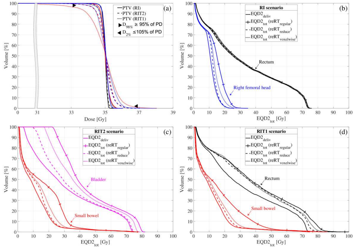
Figure 3. Dose-volume histograms (DVHs) using dose and total equivalent dose in 2-Gy fraction (EQD2 tot ) for the three relapse scenarios – repeat irradiation (RI), re-irradiation type 1 (RIT1) and type 2 (RIT2). (a): DVHs for the planning target volumes (PTV) with a broken x-axis for reRT regular (black lines), reRT reduce (red lines) and reRT voxelwise (blue lines) for all three relapse scenarios with the PTV coverage goals marked as horizontal black triangles. [(b), (c), and (d)]: DVHs of two organs at risk per relapse scenario for the first treatment course (EQD2 deliv ) in full lines and the EQD2 tot for reRT regular (full lines with perpendicular crossing lines), reRT reduce (dashed lines) and reRT voxelwise (dotted lines). (b): The RI scenario, (c): the RIT2 scenario and (d): the RIT1 scenario. The EQD2 was calculated using an \alpha/\beta = 3 Gy for all voxels.
