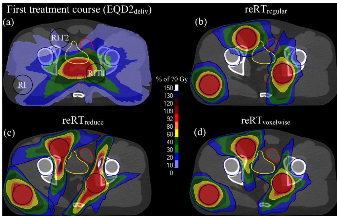
Figure 2. (a): The equivalent dose in 2-Gy fraction (EQD2) distribution of the first treatment course (EQD2 deliv ) with the three fictitious relapse planning target volumes (PTVs) marked in black; RI (repeat irradiation), RIT1 (re-irradiation type 1) and RIT2 (re-irradiation type 2). The superimposed EQD2 distributions for the three relapse scenarios are shown for (b) reRT regular , (c) reRT reduce and (d) reRT voxelwise . The EQD2 was truncated at 14 Gy (20% iso-EQD2 line) to avoid overlap, leaving only a minor overlap of the 20% iso-EQD2 line of RI and RIT2 in (c). The contours of bladder, rectum, small bowel, and femoral heads are marked in yellow, brown, red, and blue, respectively. The EQD2 distributions were calculated using an \alpha/\beta = 3 Gy for all voxels. 92% and 109% of 70 Gy EQD2 approximately corresponds to 95% and 105% of 35 Gy in 5 fractions, respectively.
