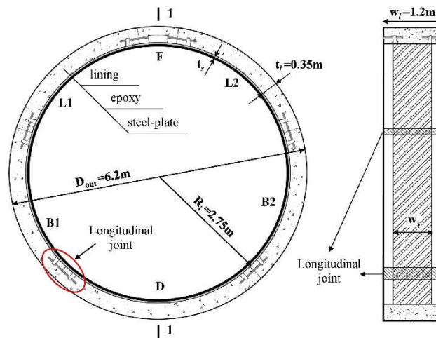
Fig. 34. Bonded steel plate method [127].
