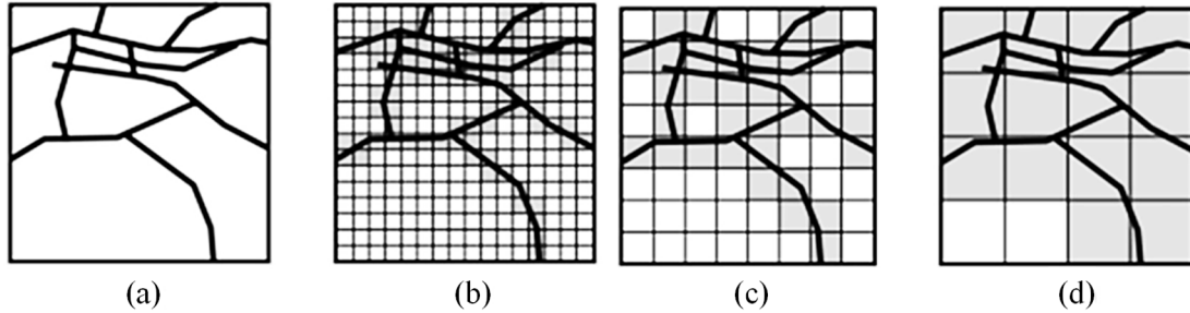
Fig. 28. Schematic diagram of the Box-Counting method. (a) Crack image; (b) r = 1, N(r) = 86 ; (c) r = 2, N(r) = 34 ; (d) r = 4, N(r) = 14 [25].
