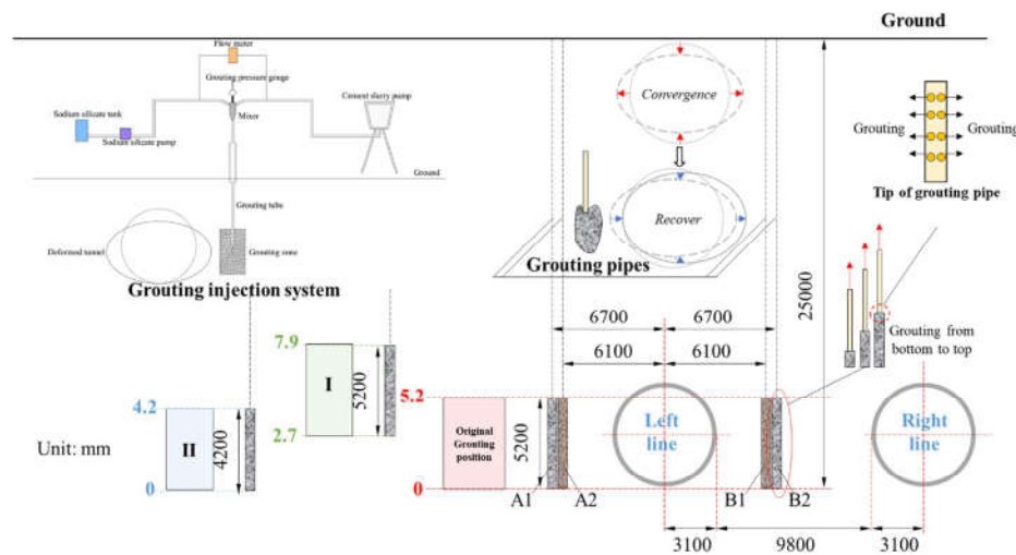
Fig. 39. The grouting system and working procedure [170].
