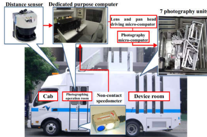
Fig. 12. The tunnel lining surface photography vehicle components [25].
