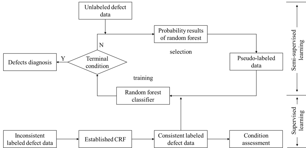
Fig. 32. Schematic illustration of the cloud model-based random forests [30].
