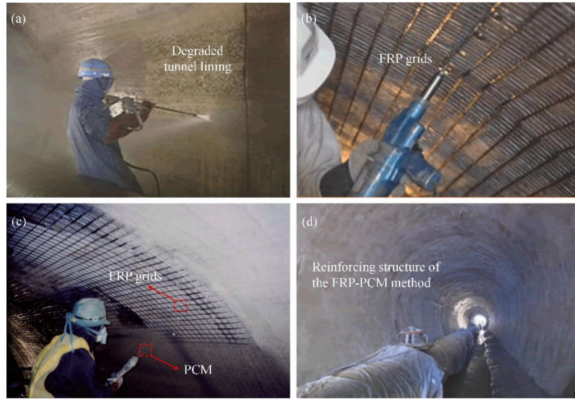
Fig. 38. Application of the FRP-PCM method on tunnel linings: (a) surface treatment; (b) fix the FRP grids; (c) spray the PCM; (d) after the construction [161].
