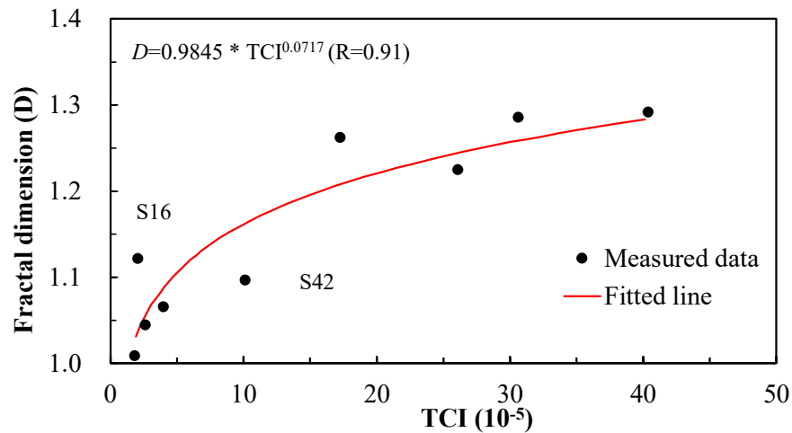
Fig. 29. Correlation between fractal dimension and TCI [25].
