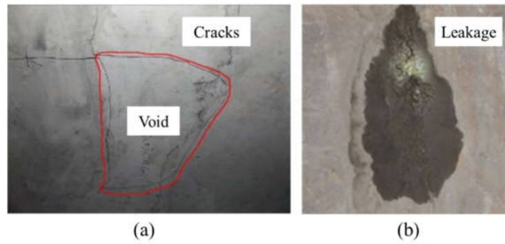
Fig. 1. Typical tunnel lining defects: (a) cracks and void [13]; (b) leakage [46].
