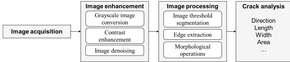
Fig. 3. Flowchart of conventional image processing.
