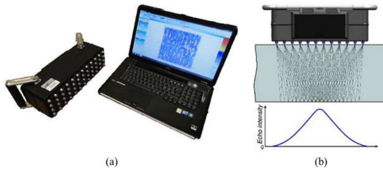
15 16 Fig. 23. (a) The A1040 MIRA system and (b) the transmission/reception of acoustic waves 17 and corresponding echo intensity [97].
