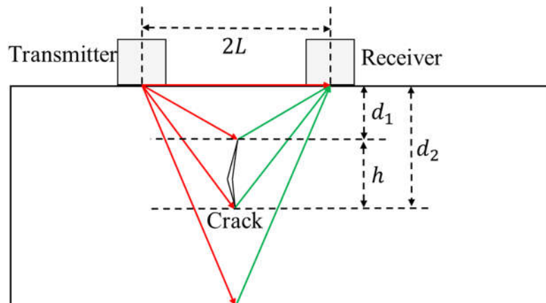
Fig. 8. Principle of TOFD.
