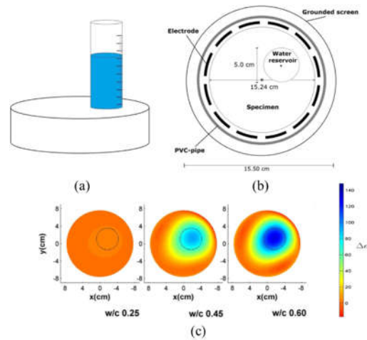
Fig. 18. ECT experiment: (a) a specimen and a water reservoir, (b) top view of the ECT experimental set-up and (c) ECT reconstructions of three specimens with different water-cement mass ratios after 48 hours [84].
