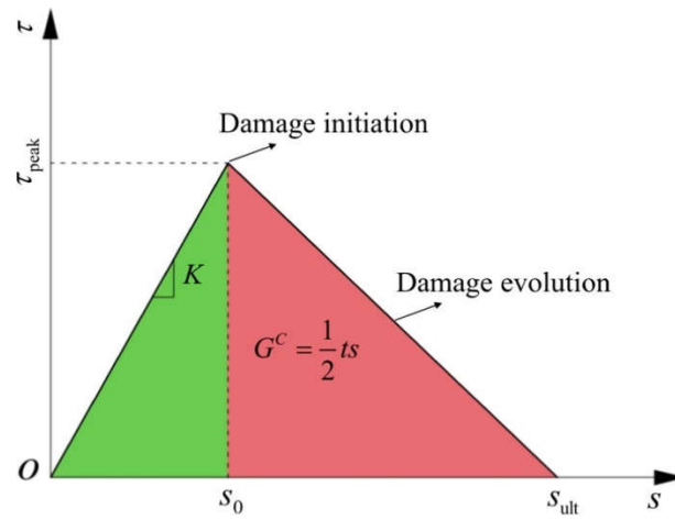
Fig. 36. A model for bond damage evolution based on traction separation response [139].
