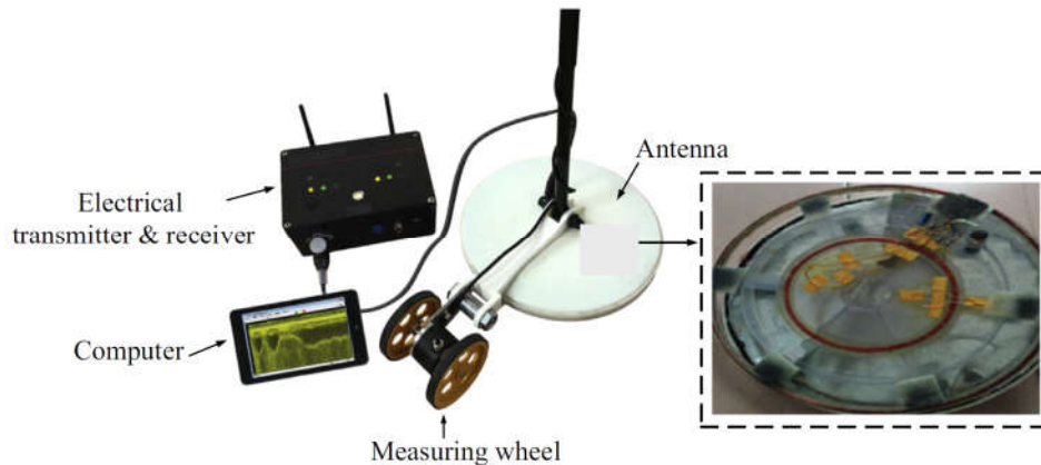
Fig. 22. TER system components [91].
