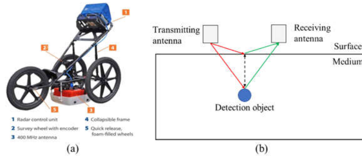
Fig. 6. (a) The GPR radar GSSI SIR 3000 and (b) principle of GPR [57].
