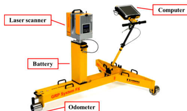
Fig. 17. The MLS system GRP5000 [80].
