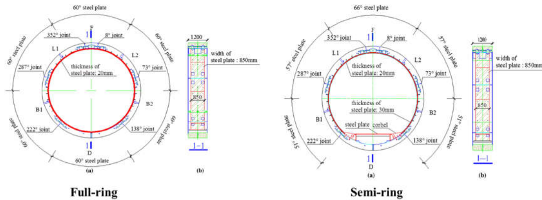
Fig. 35. Shield tunnel reinforced by steel plate: (a) cross-section; (b) longitudinal section [129].
