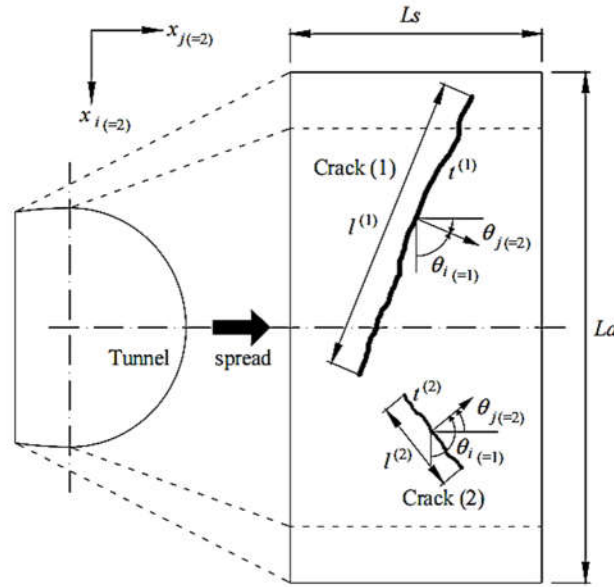
Fig. 27. The conceptual diagram of TCI [29].
