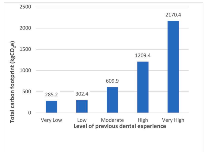
Fig. 4. Total carbon footprint from patients with different levels of previous dental disease and treatment experience.
