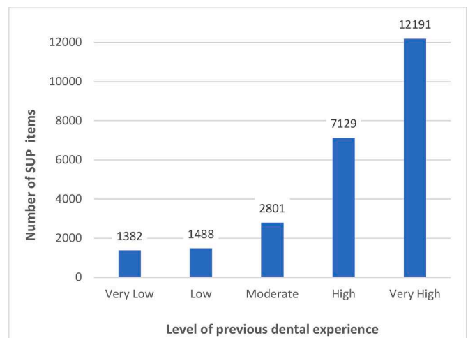
Fig. 5. Total number of Single Use Plastics (SUPs) used for treatment in patients with different levels of previous dental disease and treatment experience.
