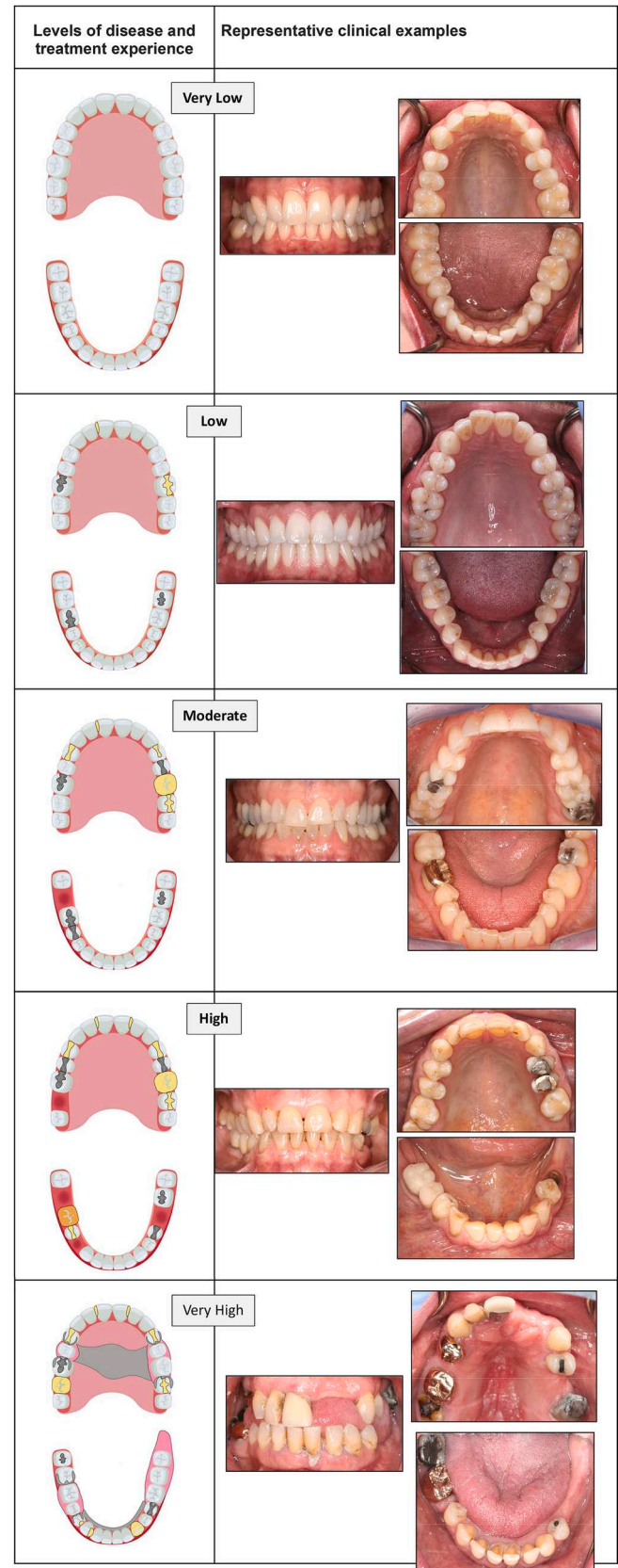
Fig. 3. Column 1: Diagrammatic representation of the different levels of disease and treatment experience identified in Table 1 and depicted in Fig. 2. Column 2: Representative clinical examples of previous levels of previous dental disease and treatment experience.
