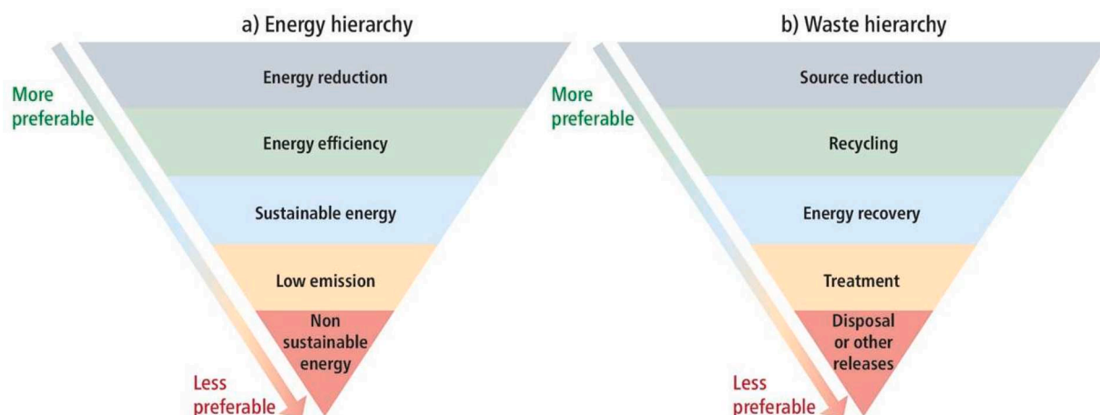
Fig. 1. Inverted pyramids for energy and waste hierarchies. First published in 'SDG 7: affordable and clean energy in oral healthcare' British Dental Journal, Vol 235, 454–455, 2023 by Springer Nature.
