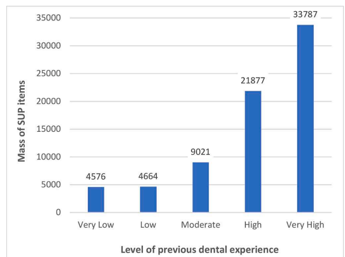
Fig. 6. Total weight of Single Use Plastics (SUPs) used for treatment in patients with different levels of previous dental disease and treatment experience.
