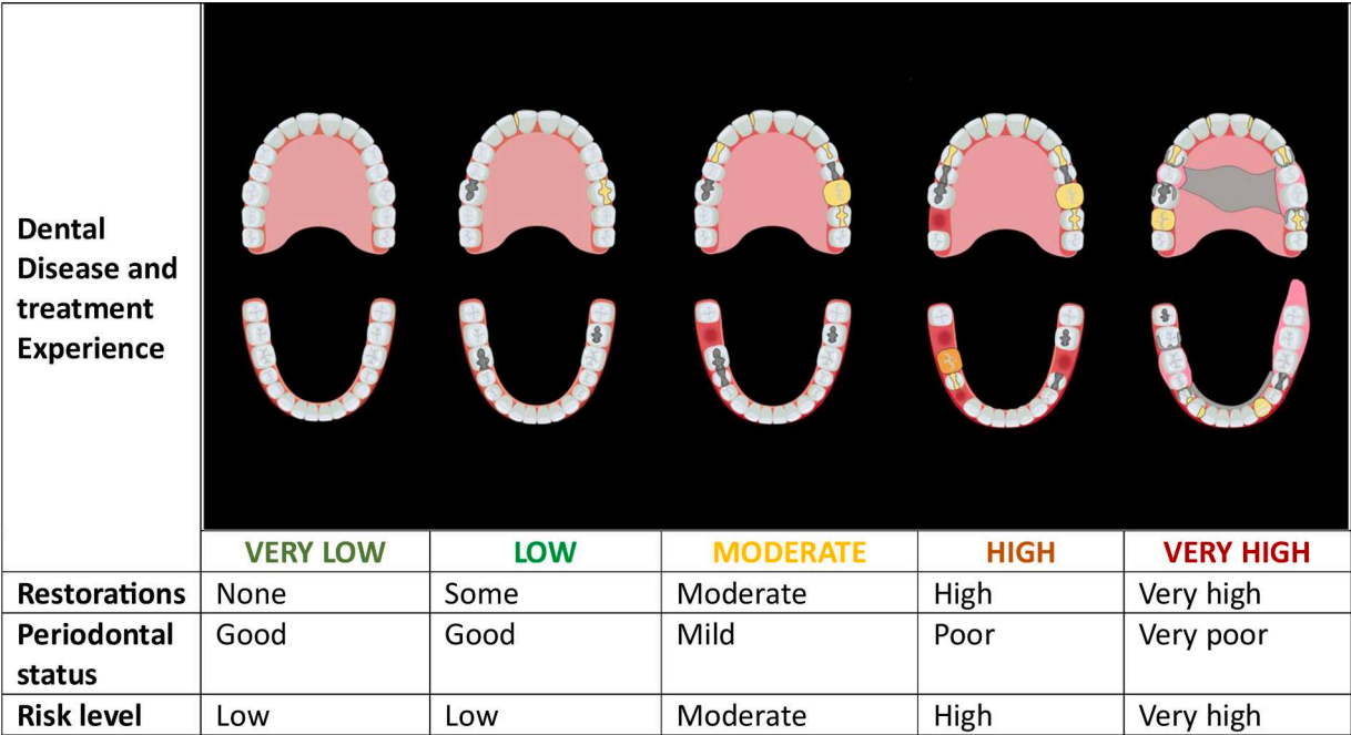
Fig. 2. Diagrammatic representation of the previous levels of dental disease and treatment experience, mapped to Table 1.
