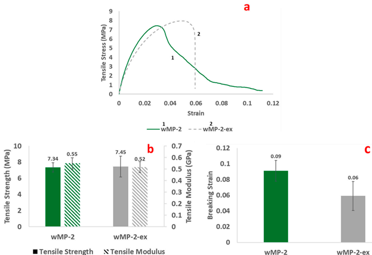
Figure 10. (a) Representative tensile stress–strain curves, (b) tensile strength and tensile modulus, and (c) breaking strain of wMP manufactured with different processing methods.
