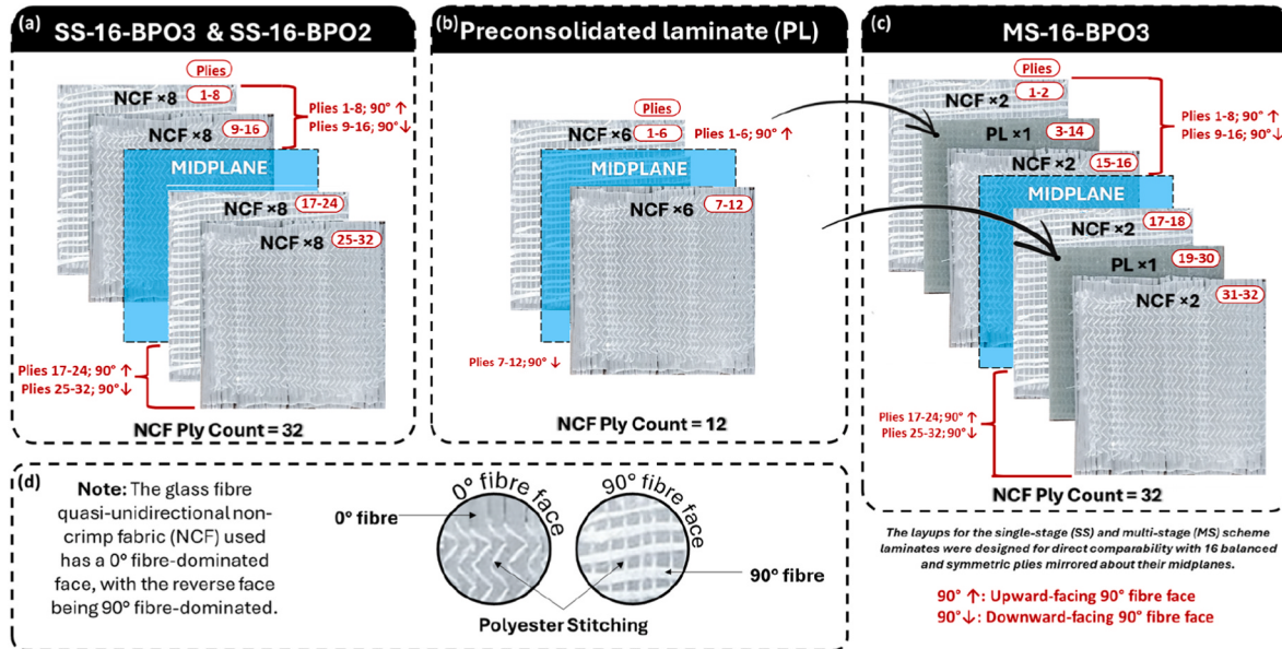
Fig. 2. Illustrative representation of the balanced and symmetric layup adopted to match the 16-mm-thick laminates produced using single-stage (SS-16-BPO3 and SS-16-BPO2) and multi-stage (MS-16-BPO3) schemes for direct comparability.
