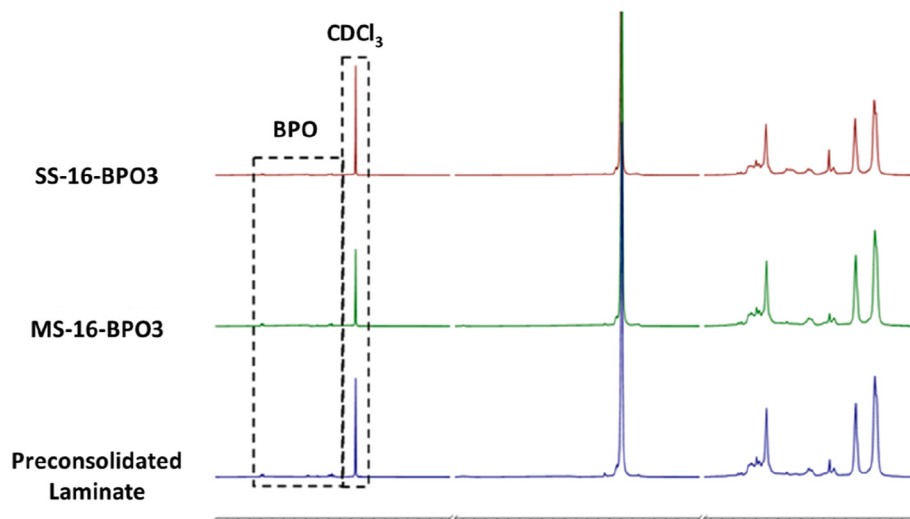
Fig. 5. 1 H NMR spectra of recovered polymer matrices in chloroform. Note: Samples are from the SS-16-BPO3, MS-16-BPO3 and 6-mm-thick preconsolidated laminates (PL). The MS-16-BPO3 was produced with two pieces of the PL as inserts as part of the additive-free exothermic control scheme under investigation.
