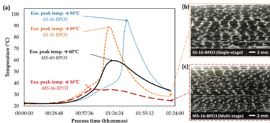
Fig. 3. (a) Liquid resin infusion and in-situ polymerisation thermal profiles were recorded using a TC-08 thermocouple data logger with a mid-plane embedded k-type thermocouple at room temperature. Exothermic peak temperatures are annotated for each glass fibre/acrylic laminate. (b) and (c) Comparative full-thickness, cross-sectional micrographs for SS-16-BPO3 and MS-16-BPO3 laminates, respectively.
