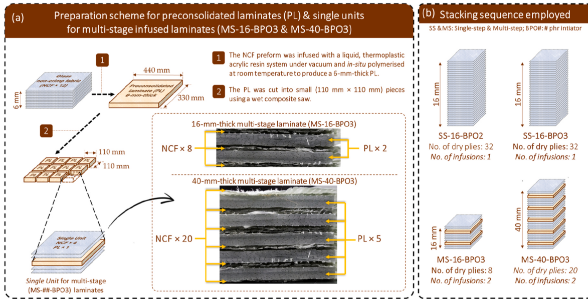
Fig. 1. Graphical representations of (a) the preparation of PL pieces for the MS-16-BPO3 and MS-40-BPO3 laminates; and (b) the stacking sequence employed for the SS-16-BPO2, SS-16-BPO3, MS-16-BPO3, and MS-40-BPO3 laminates. Note: All laminates were manufactured using a liquid resin infusion method at room temperature under vacuum. SS, MS, BPO, NCF, and PL stand for single-stage, multi-stage, benzoyl peroxide initiator, non-crimp fabric, and preconsolidated laminate, respectively. The suffixes -BPO2 and -BPO3 indicate the initiator contents, i.e., 2 phr or 3 phr, respectively.
