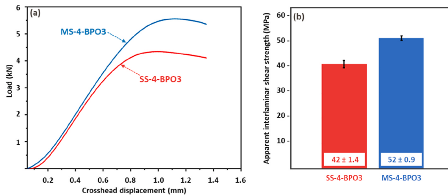
Fig. 6. (a) Representative short beam shear load-displacement curves and (b) mean apparent interlaminar shear strengths for 4-mm-thick test laminates SS-4-BPO3 and MS-4-BPO3, produced using single- and multi-stage resin infusion scheme, respectively.
