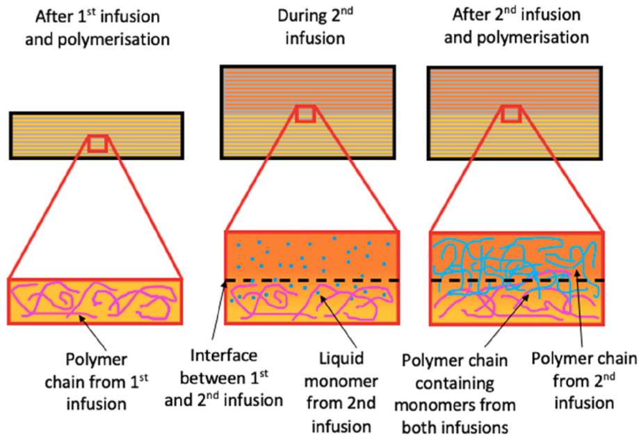
Fig. 4. A schematic showing the formation of a semi-IPN at the joining plane within the multi-stage resin-infused and in-situ polymerised laminates.
