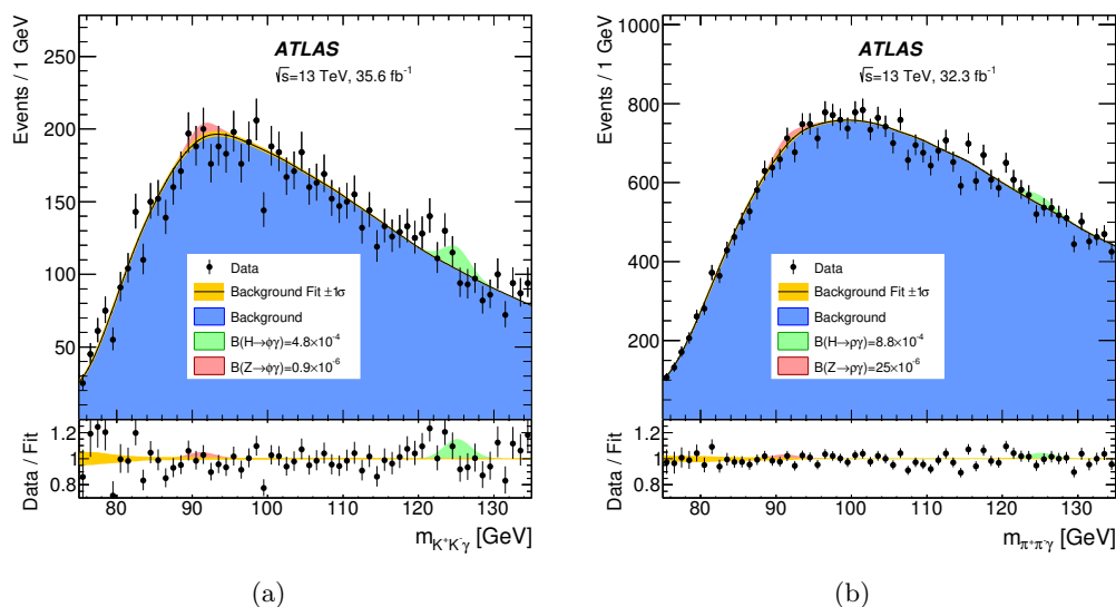
Figure 5. The (a) m_{K+K-\gamma} and (b) m_{\pi+\pi-\gamma} distributions of the selected \phi\gamma and \rho\gamma candidates, respectively, along with the results of the maximum-likelihood fits with a background-only model. The Higgs and Z boson contributions for the branching fraction values corresponding to the observed 95% CL upper limits are also shown. Below the figures the ratio of the data to the background-only fit is shown.
