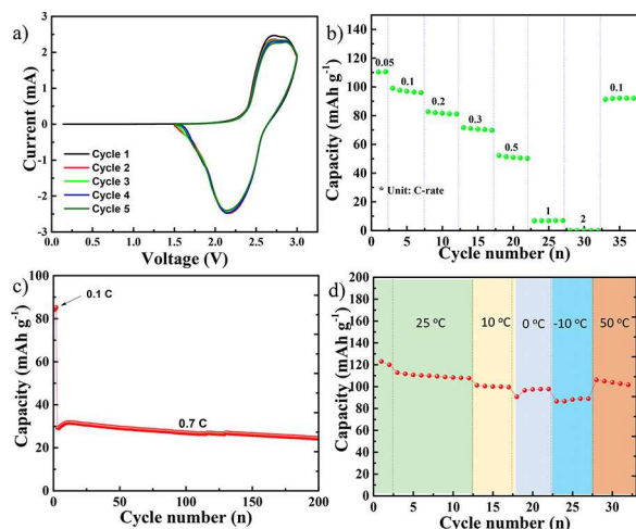
Figure 5. (a) Cyclic voltammetry at a scan rate of 0.2 mV s -1 , (b) rate performance, (c) cycling performance, and (d) cycling performance at different ambient temperatures at a current rate of 0.2C of the LMO/LTO all dry full cell.
