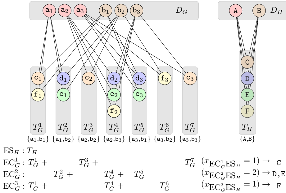
Fig. 2. A locally bijective homomorphism from a graph G (left) to a graph H (right), augmenting the partial homomorphism \phi_P mapping the vertices of the vertex cover D_G into D_H = \{A, B\} . The i th vertex of G mapped to some vertex X of H is denoted x_i . Vertices in G \setminus D_G are grouped by type (e.g. \{c_1\} and \{f_1\} have type T_G^1 ), each T_G^i is characterised by the neighbours of its vertices, recalled below each column. Vertices in H \setminus D_H all have the same type T_H . Rows EC_G^i are extensions that can be minimally \phi_P -B-mapped to T_H . This, in particular, means that each a_i and b_i must have a neighbour in EC_G^i . This is because otherwise a_i or b_i is not mapped locally bijective to its image A or B , because A and B have a neighbour in T_H , but the particular a_i or b_i has no neighbour in EC_G^i . Note that the neighbour can then later be used as a pre-image of any vertex in \{C, D, E, F\} . Using EC_G^1 once (for colour C), EC_G^2 twice (for colours D and E) and EC_G^3 once (for colour F) yields the given locally bijective homomorphism, and it can be verified that each a_i and b_i indeed has all four colours in its neighbourhood.
